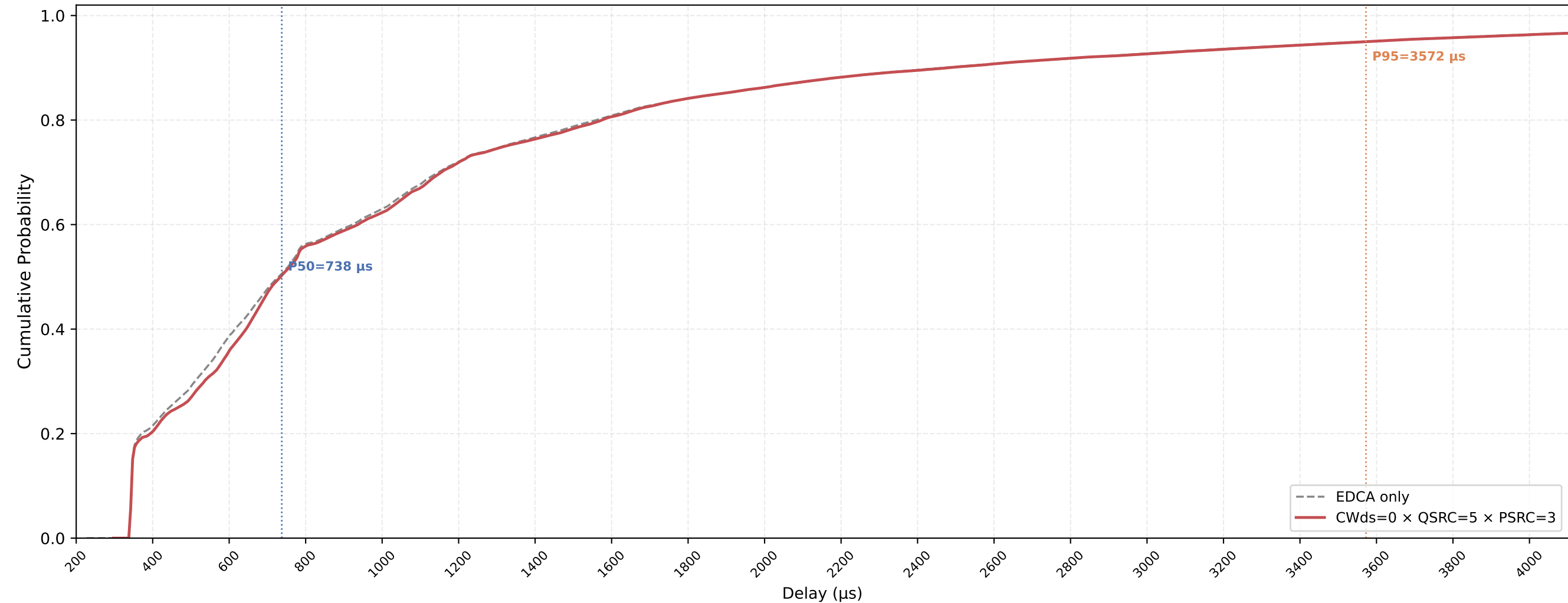
Legacy STA VO Delay CDF — CWds=0 × QSRC=5 × PSRC=3 nSta=30, nPedca=15, 0.5Mbps, avg of 10 runs
