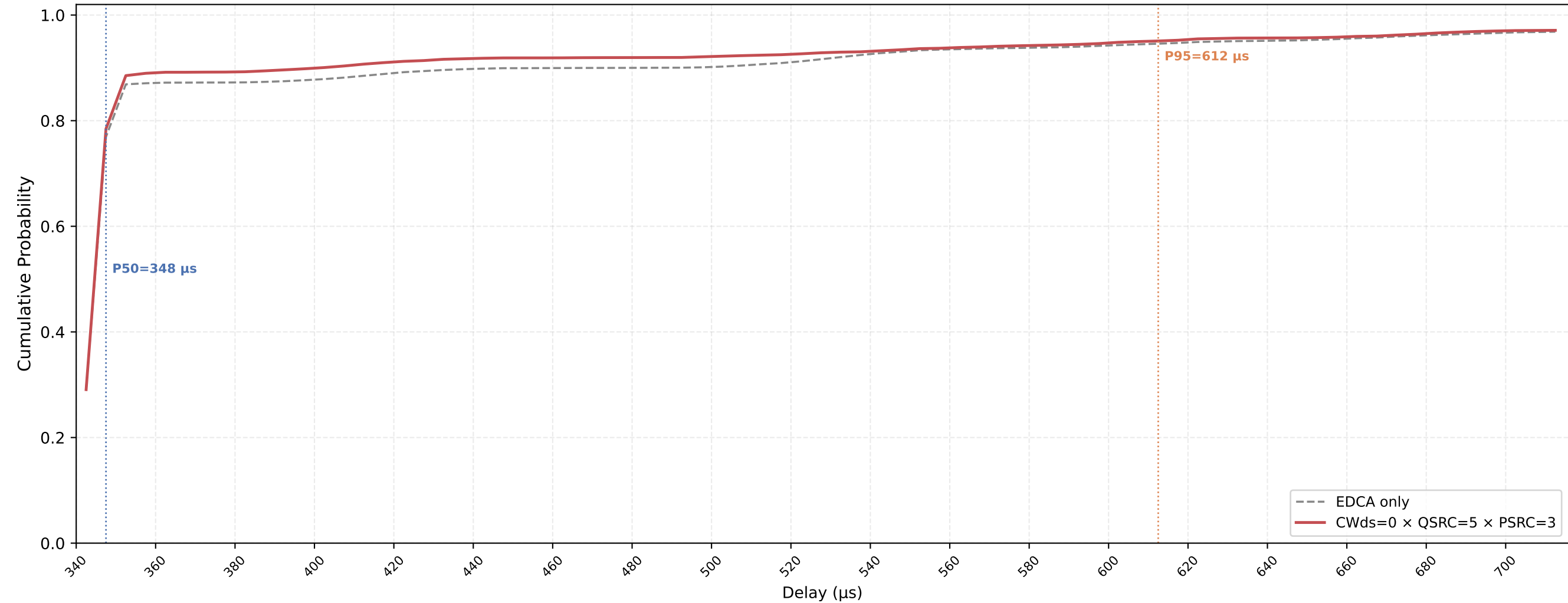
P-EDCA STA VO Delay CDF — CWds=0 × QSRC=5 × PSRC=3 nSta=30, nPedca=15, 0.1Mbps, avg of 10 runs
