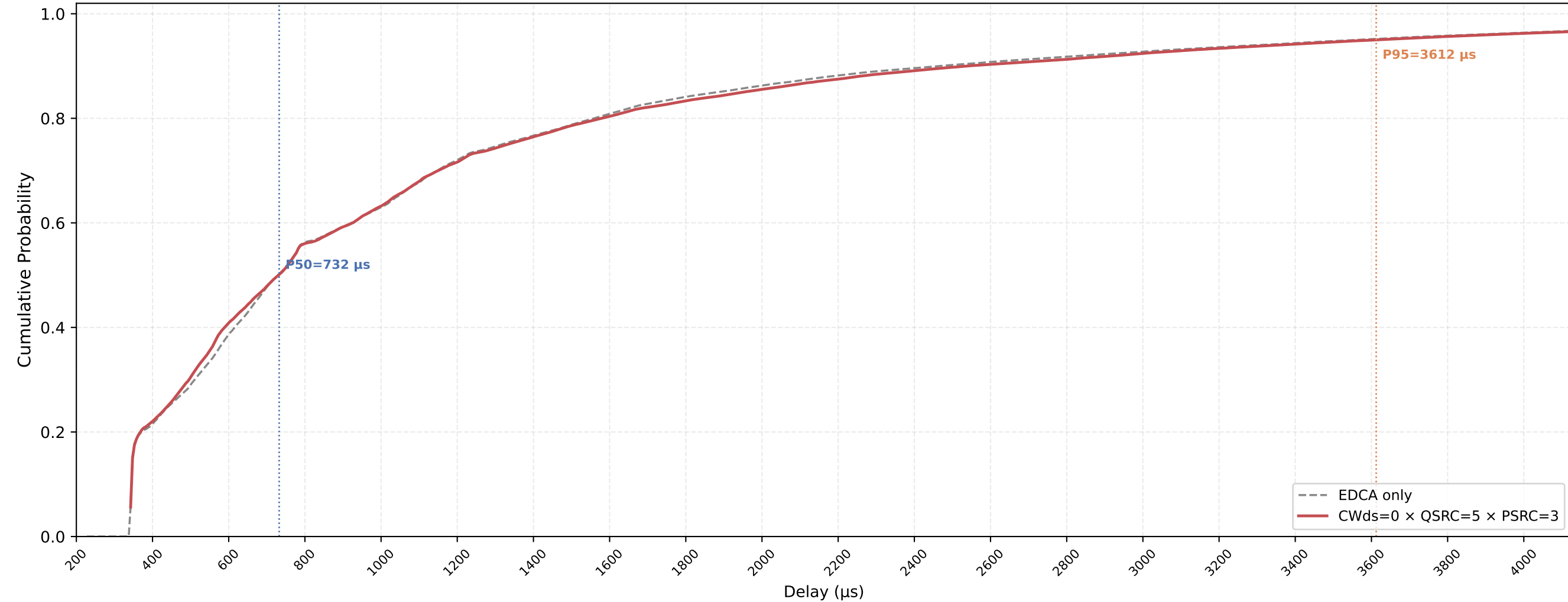
P-EDCA STA VO Delay CDF — CWds=0 × QSRC=5 × PSRC=3 nSta=30, nPedca=15, 0.5Mbps, avg of 10 runs
