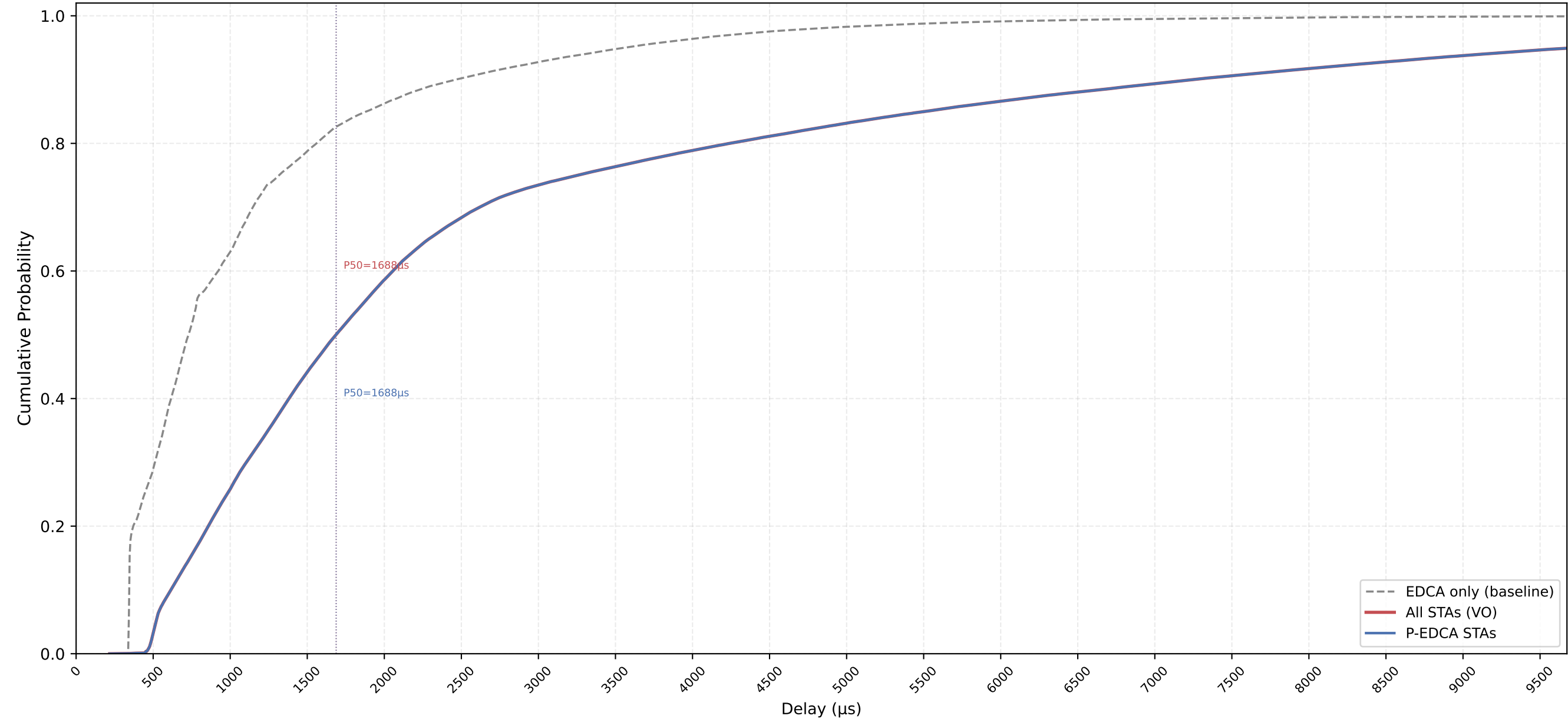
VO Delay CDF — P-EDCA / Legacy / All | CWds=1 × QSRC=0 × PSRC=1 nSta=30, nPedca=30/30, 0.5Mbps, avg of 10 runs
