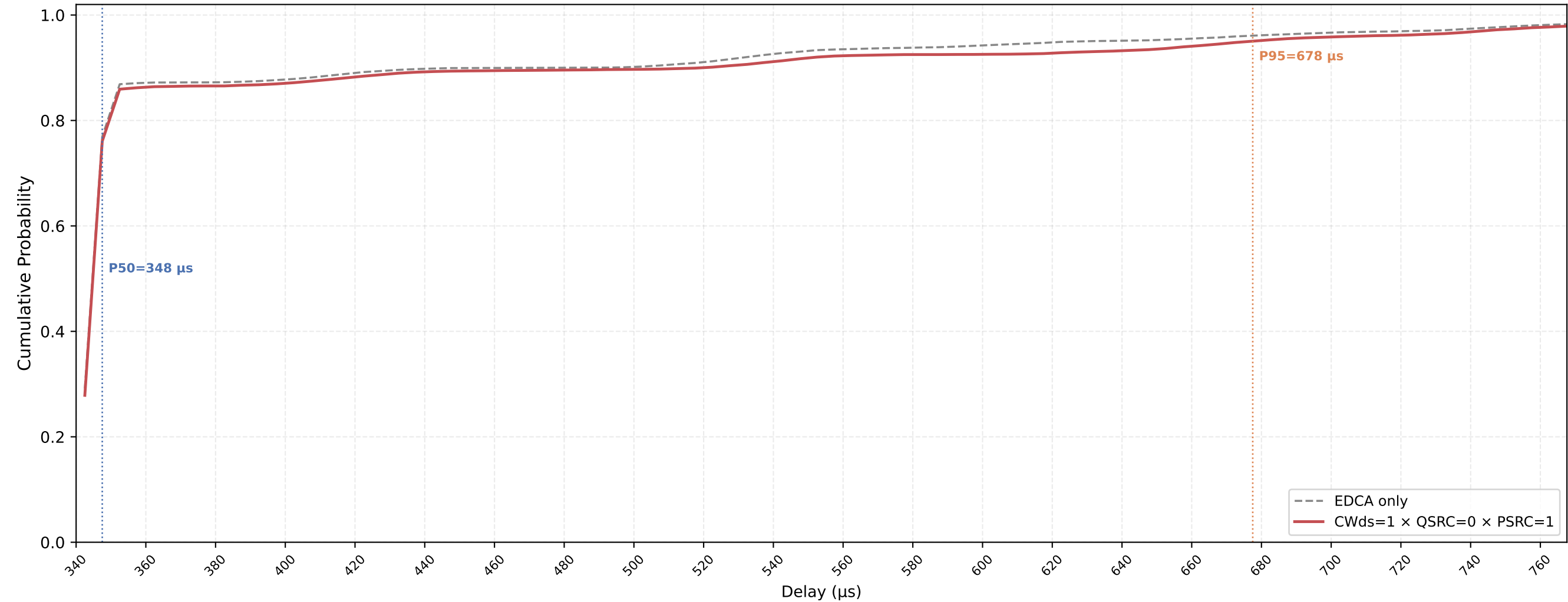
Legacy STA VO Delay CDF — CWds=1 × QSRC=0 × PSRC=1 nSta=30, nPedca=5, 0.1Mbps, avg of 10 runs
