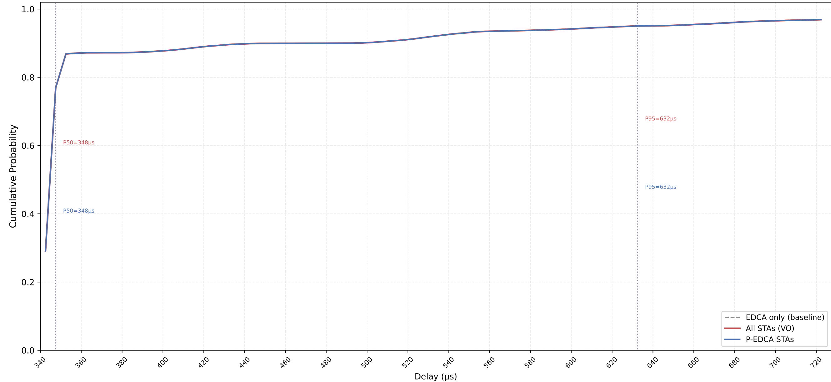
VO Delay CDF — P-EDCA / Legacy / All | CWds=1 × QSRC=1 × PSRC=1 nSta=30, nPedca=30/30, 0.1Mbps, avg of 10 runs
