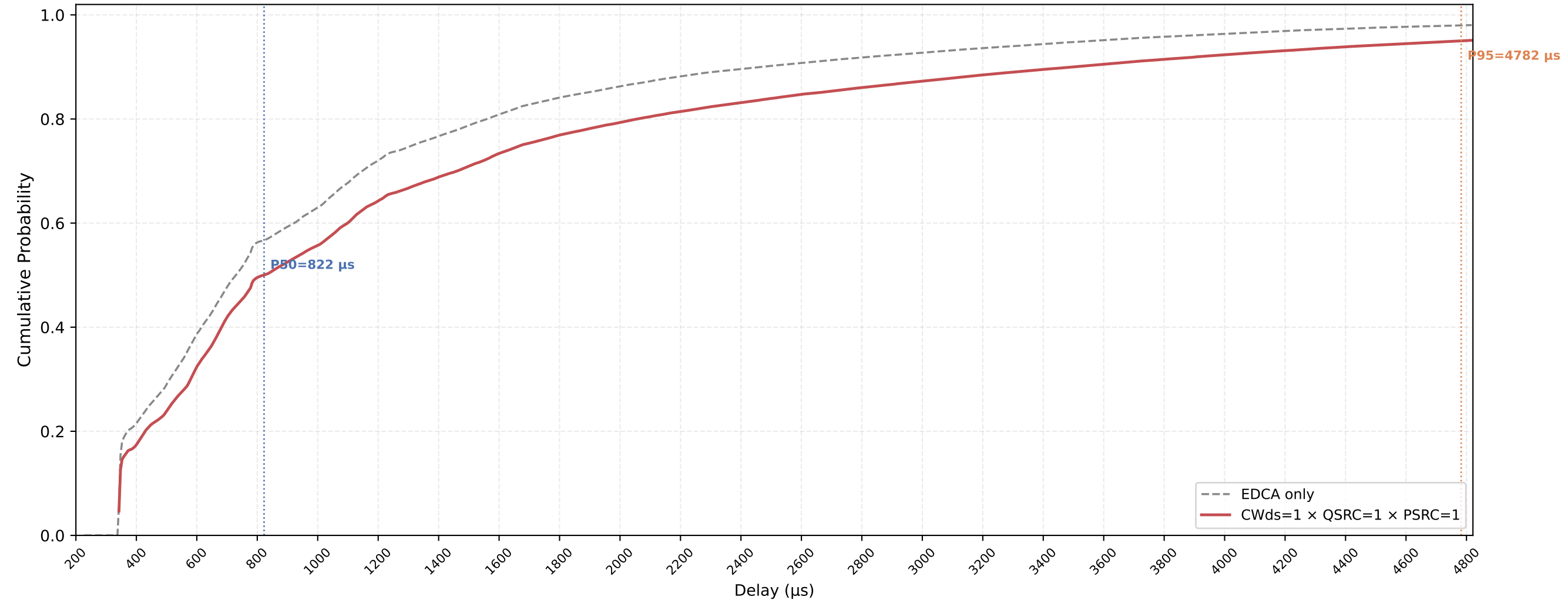
Legacy STA VO Delay CDF — CWds=1 × QSRC=1 × PSRC=1 nSta=30, nPedca=15, 0.5Mbps, avg of 10 runs
