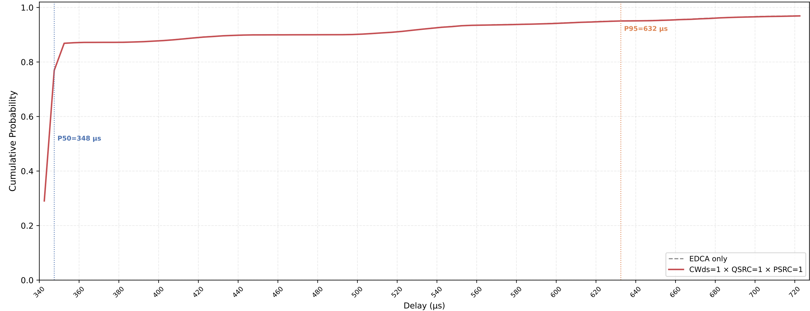
P-EDCA STA VO Delay CDF — CWds=1 × QSRC=1 × PSRC=1 nSta=30, nPedca=30, 0.1Mbps, avg of 10 runs
