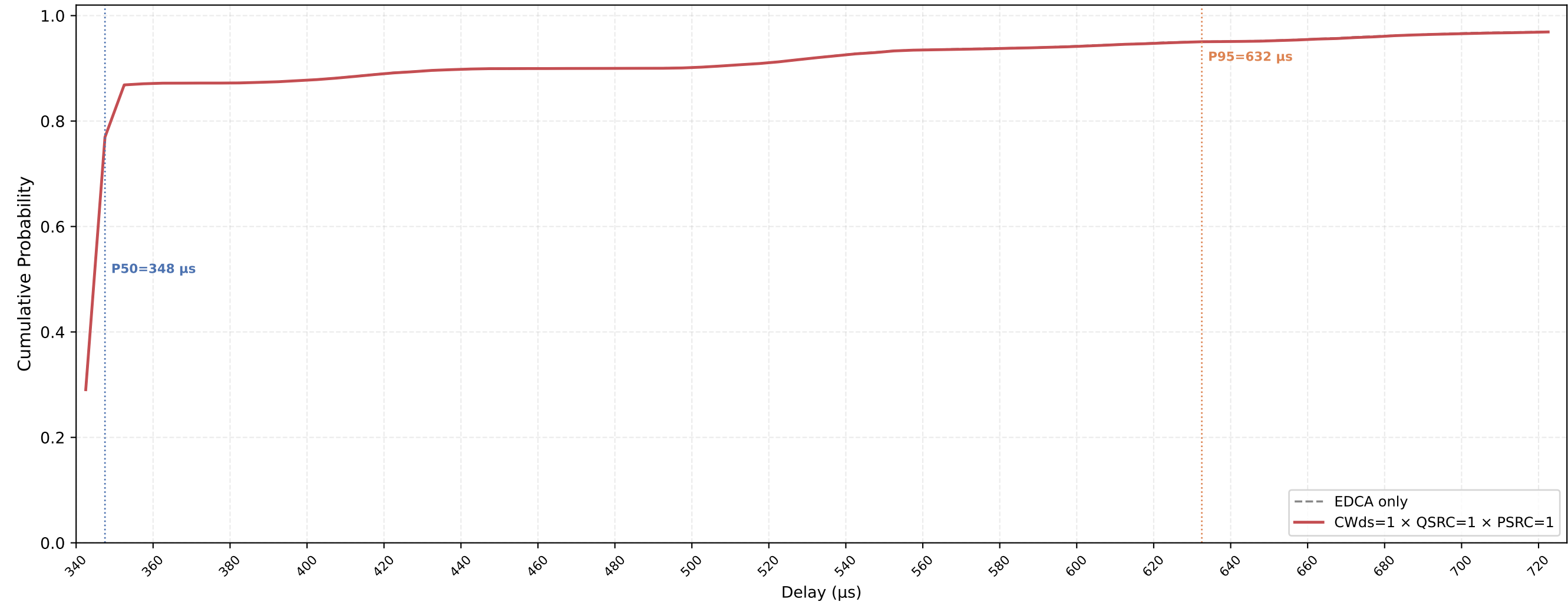
VO (all STAs) Delay CDF — CWds=1 × QSRC=1 × PSRC=1 nSta=30, nPedca=30, 0.1Mbps, avg of 10 runs
