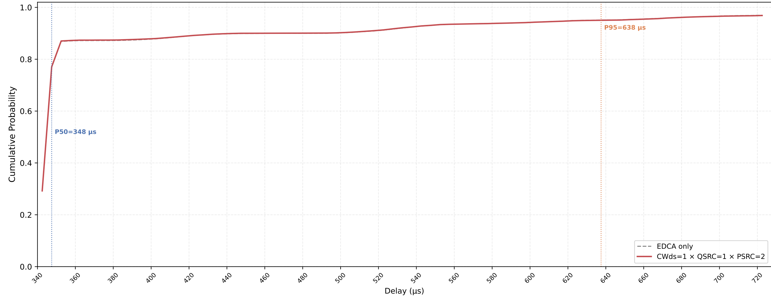
P-EDCA STA VO Delay CDF — CWds=1 × QSRC=1 × PSRC=2 nSta=30, nPedca=30, 0.1Mbps, avg of 10 runs
