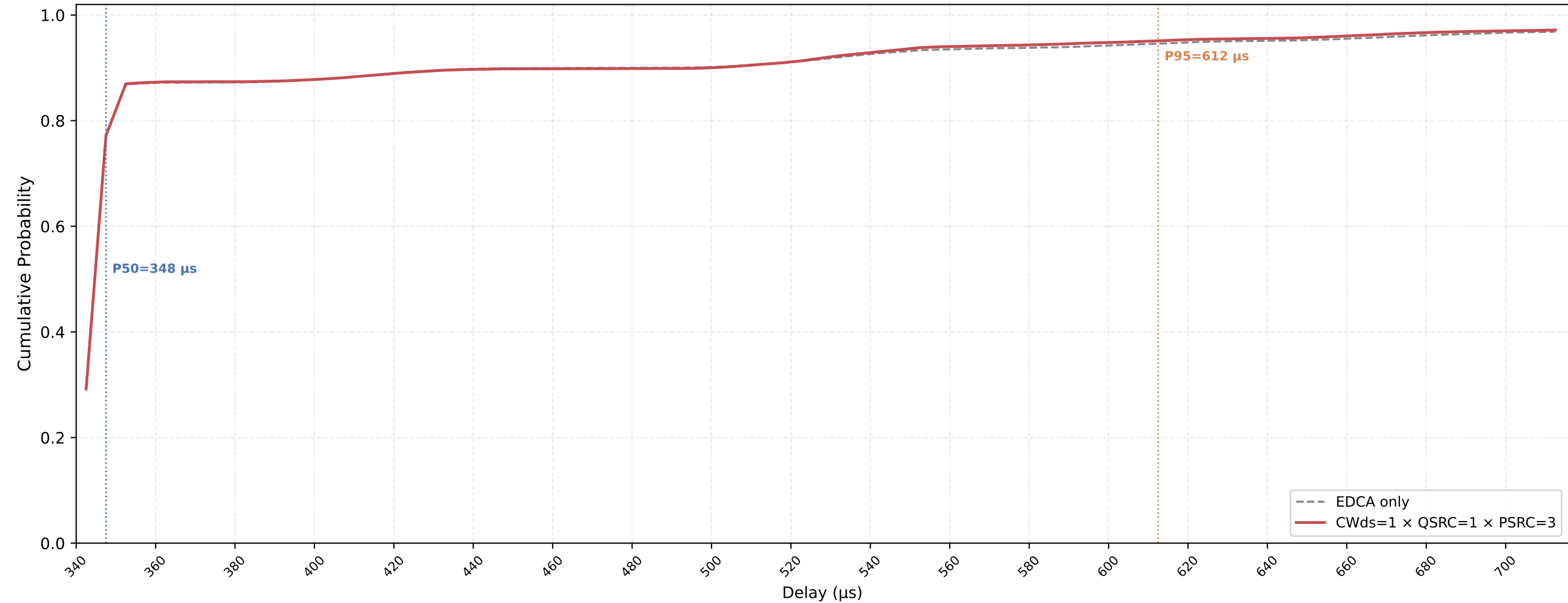
Legacy STA VO Delay CDF — CWds=1 × QSRC=1 × PSRC=3 nSta=30, nPedca=5, 0.1Mbps, avg of 10 runs
