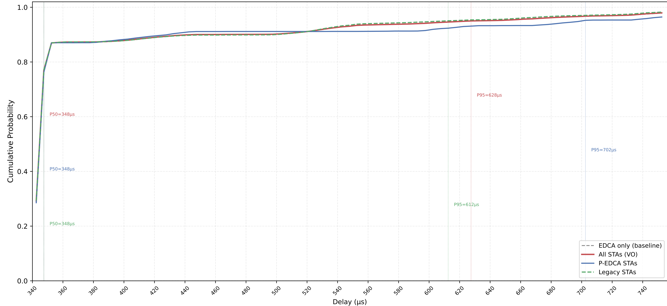
VO Delay CDF — P-EDCA / Legacy / All | CWds=1 × QSRC=2 × PSRC=1 nSta=30, nPedca=5/30, 0.1Mbps, avg of 10 runs
