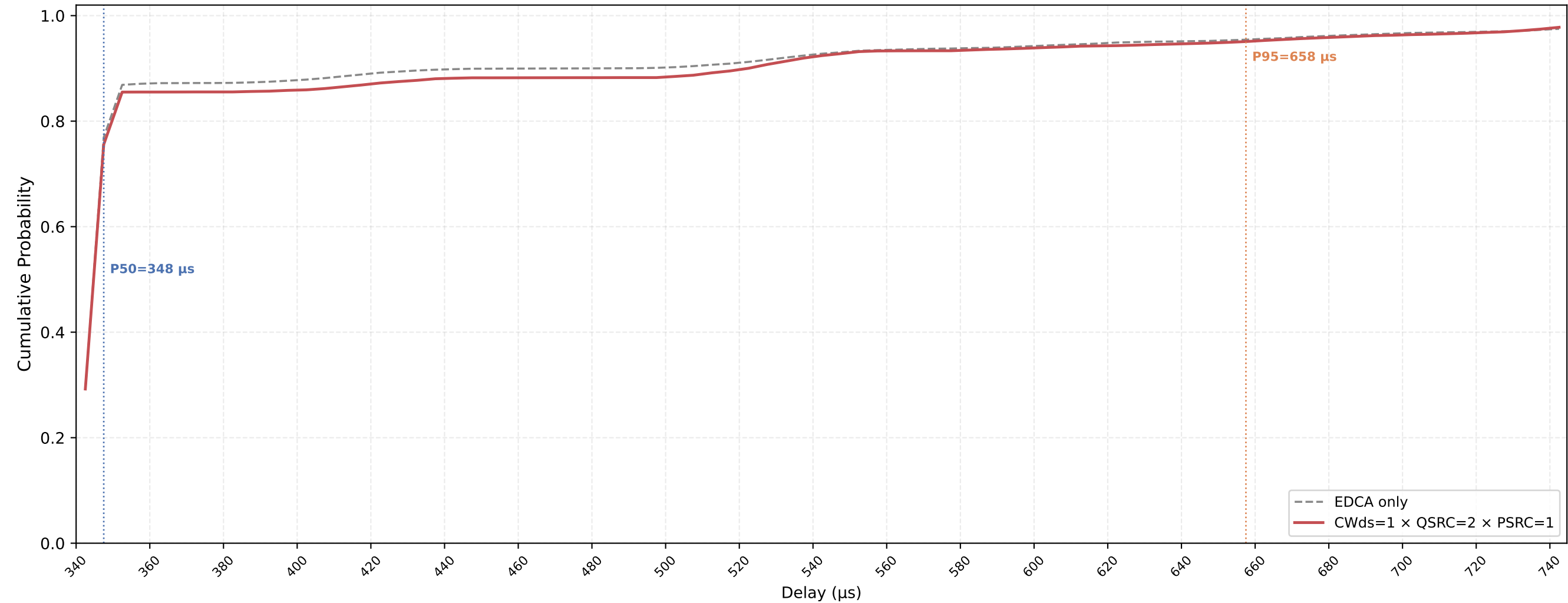
Legacy STA VO Delay CDF — CWds=1 × QSRC=2 × PSRC=1 nSta=30, nPedca=15, 0.1Mbps, avg of 10 runs
