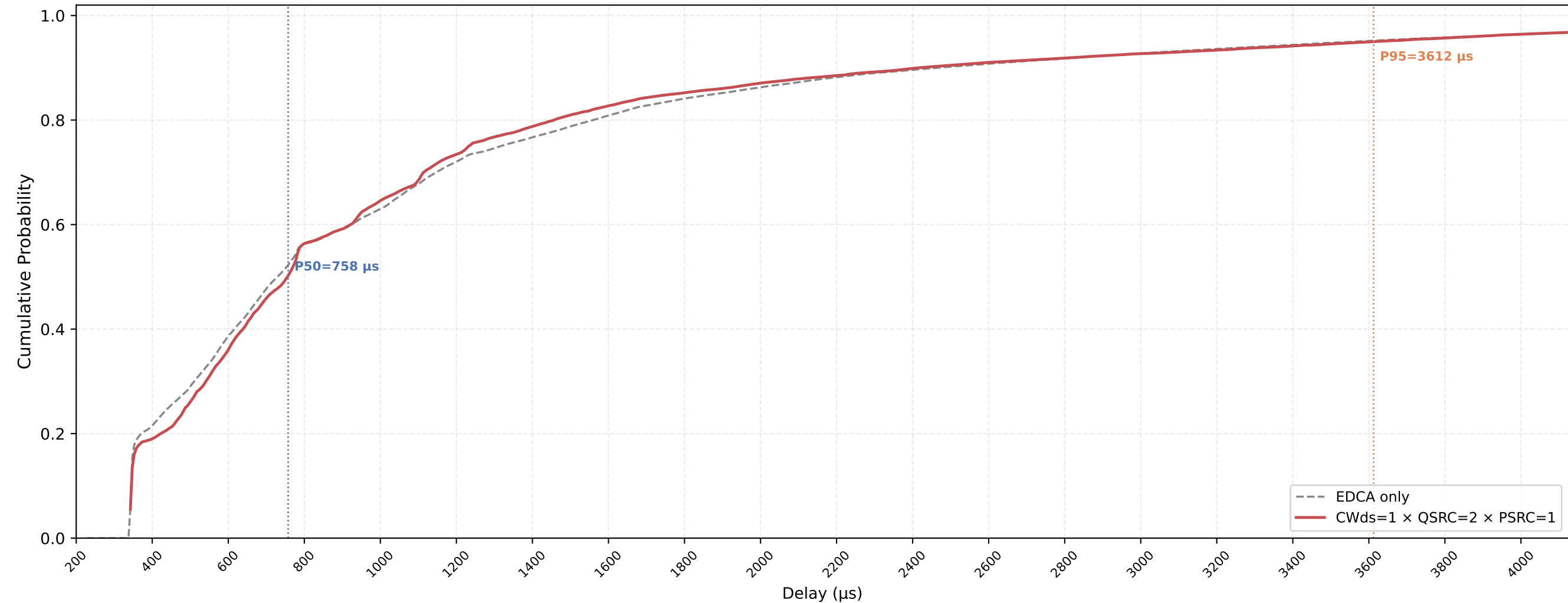
P-EDCA STA VO Delay CDF — CWds=1 × QSRC=2 × PSRC=1 nSta=30, nPedca=5, 0.5Mbps, avg of 10 runs
