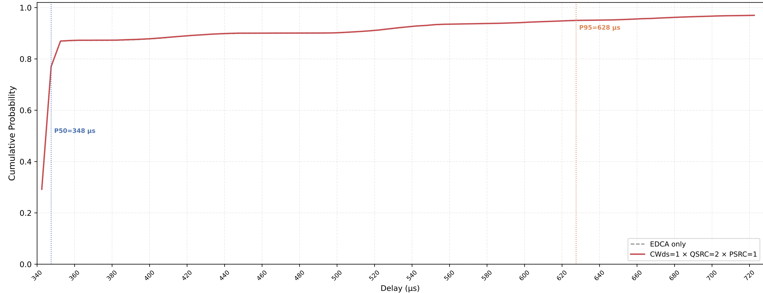
VO (all STAs) Delay CDF — CWds=1 × QSRC=2 × PSRC=1 nSta=30, nPedca=5, 0.1Mbps, avg of 10 runs
