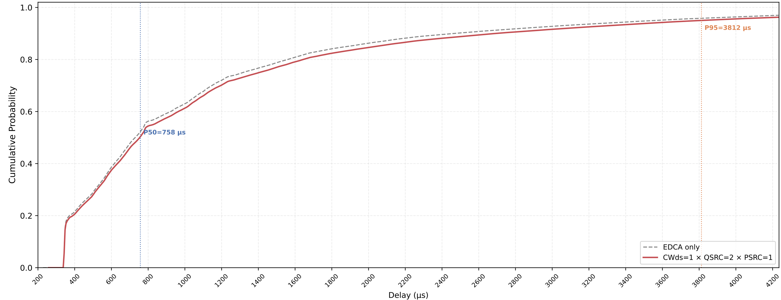
VO (all STAs) Delay CDF — CWds=1 × QSRC=2 × PSRC=1 nSta=30, nPedca=15, 0.5Mbps, avg of 10 runs
