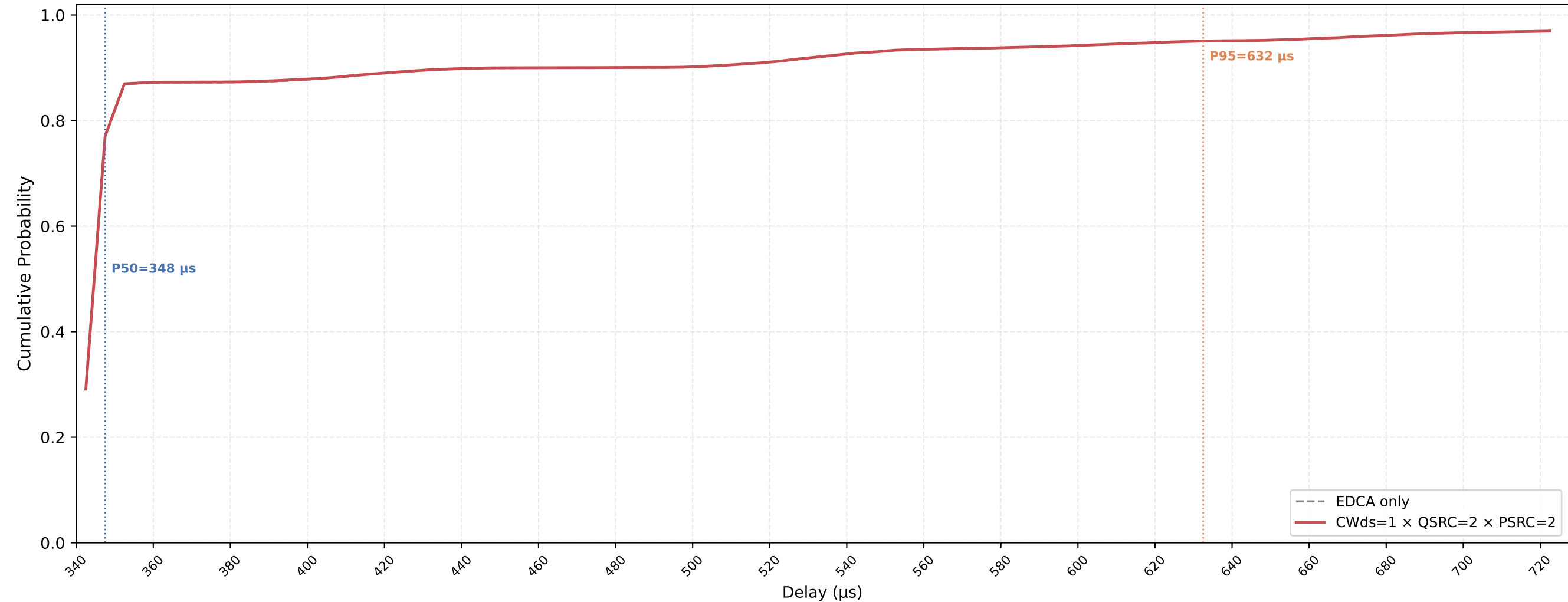
VO (all STAs) Delay CDF — CWds=1 × QSRC=2 × PSRC=2 nSta=30, nPedca=30, 0.1Mbps, avg of 10 runs
