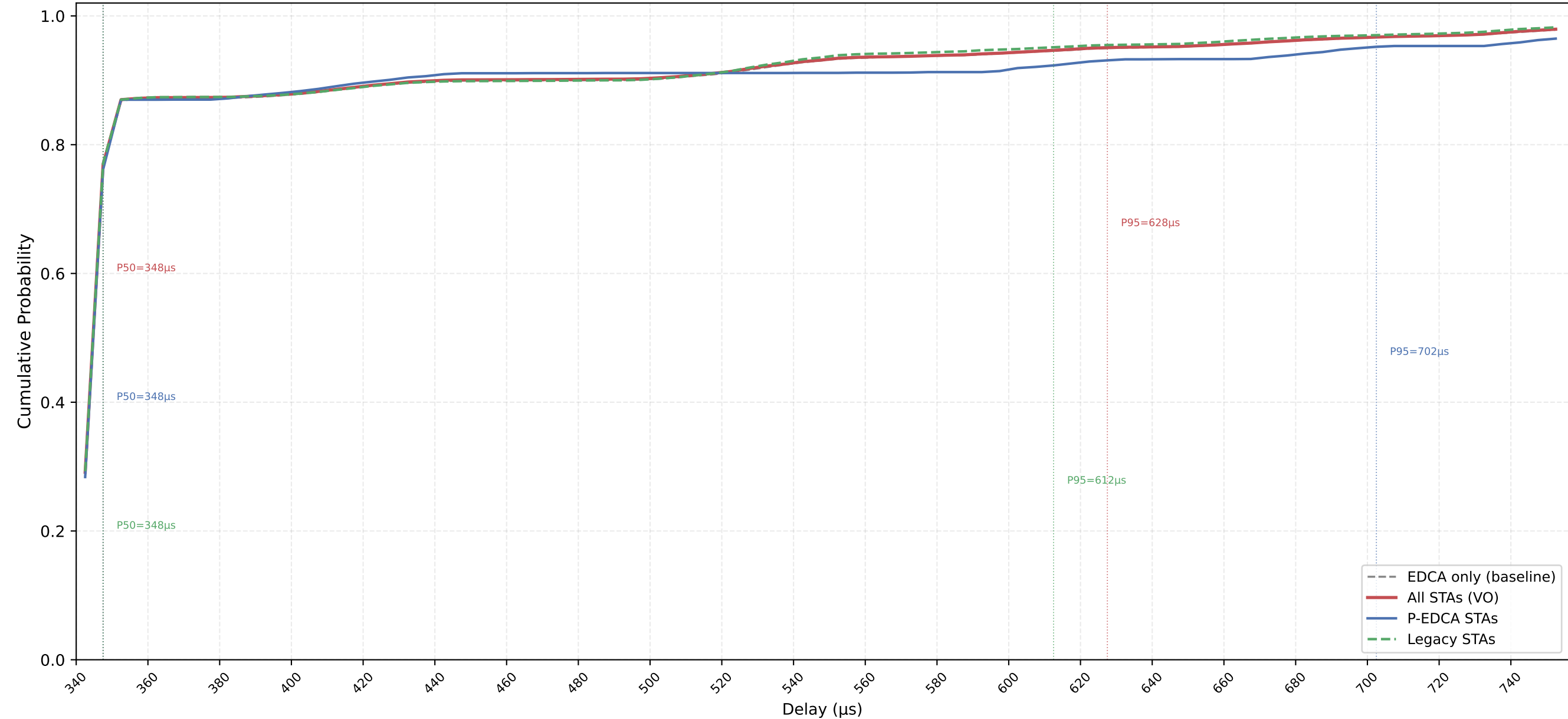
VO Delay CDF — P-EDCA / Legacy / All | CWds=1 × QSRC=2 × PSRC=3 nSta=30, nPedca=5/30, 0.1Mbps, avg of 10 runs
