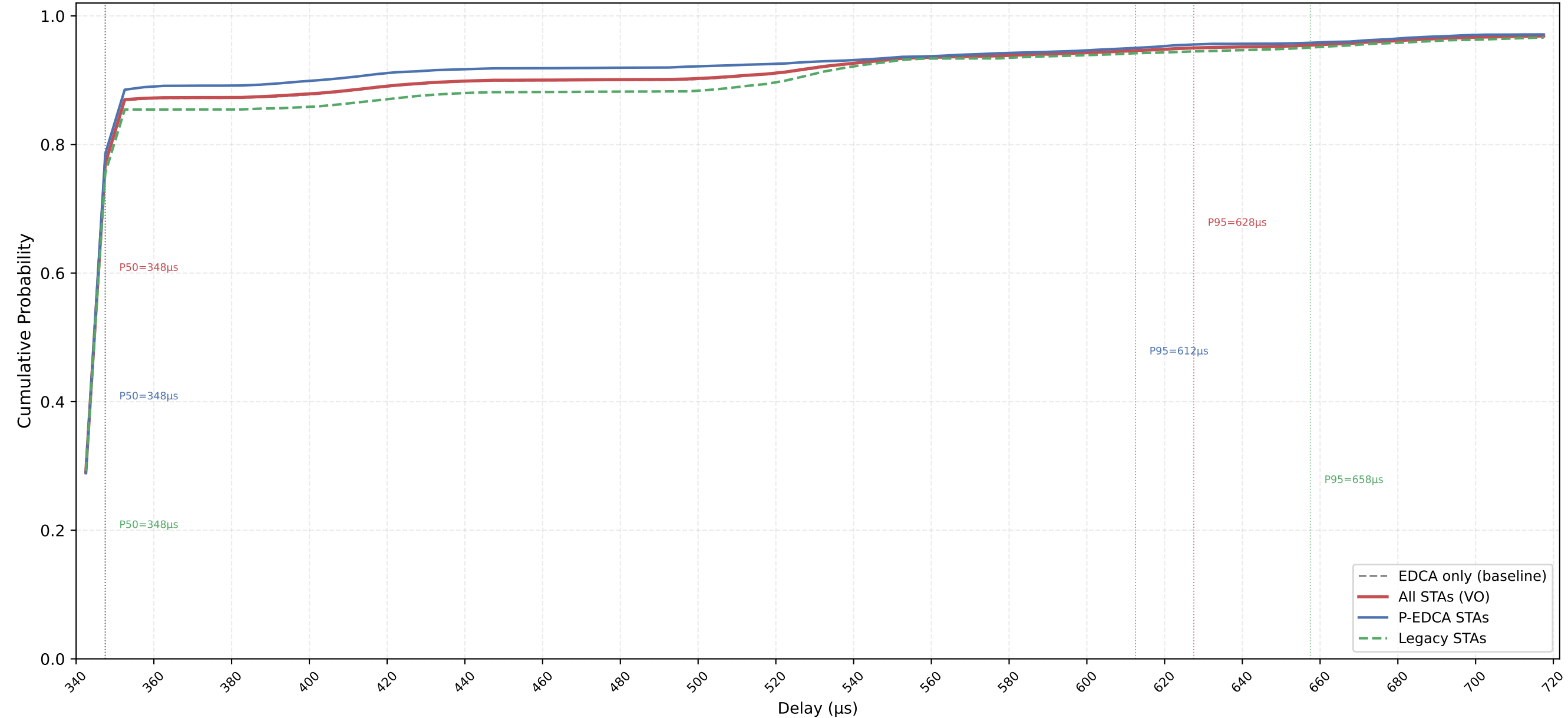
VO Delay CDF — P-EDCA / Legacy / All | CWds=1 × QSRC=2 × PSRC=3 nSta=30, nPedca=15/30, 0.1Mbps, avg of 10 runs
