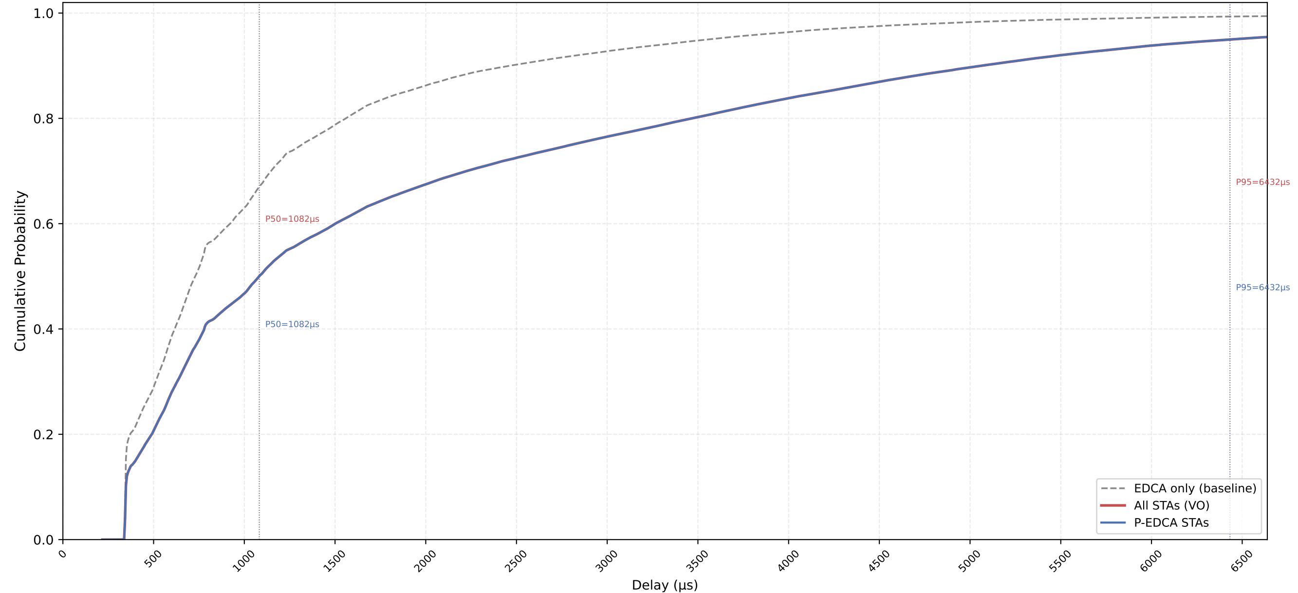
VO Delay CDF — P-EDCA / Legacy / All | CWds=1 × QSRC=2 × PSRC=3 nSta=30, nPedca=30/30, 0.5Mbps, avg of 10 runs
