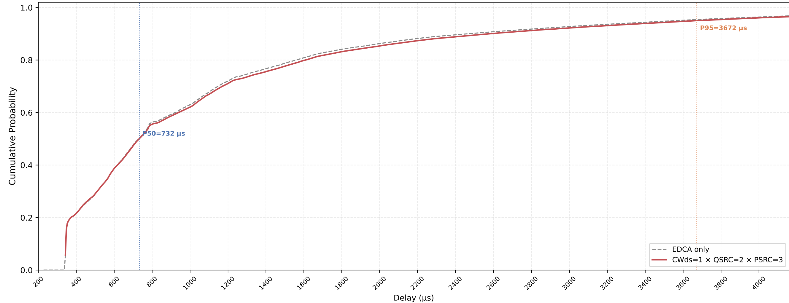
Legacy STA VO Delay CDF — CWds=1 × QSRC=2 × PSRC=3 nSta=30, nPedca=5, 0.5Mbps, avg of 10 runs
