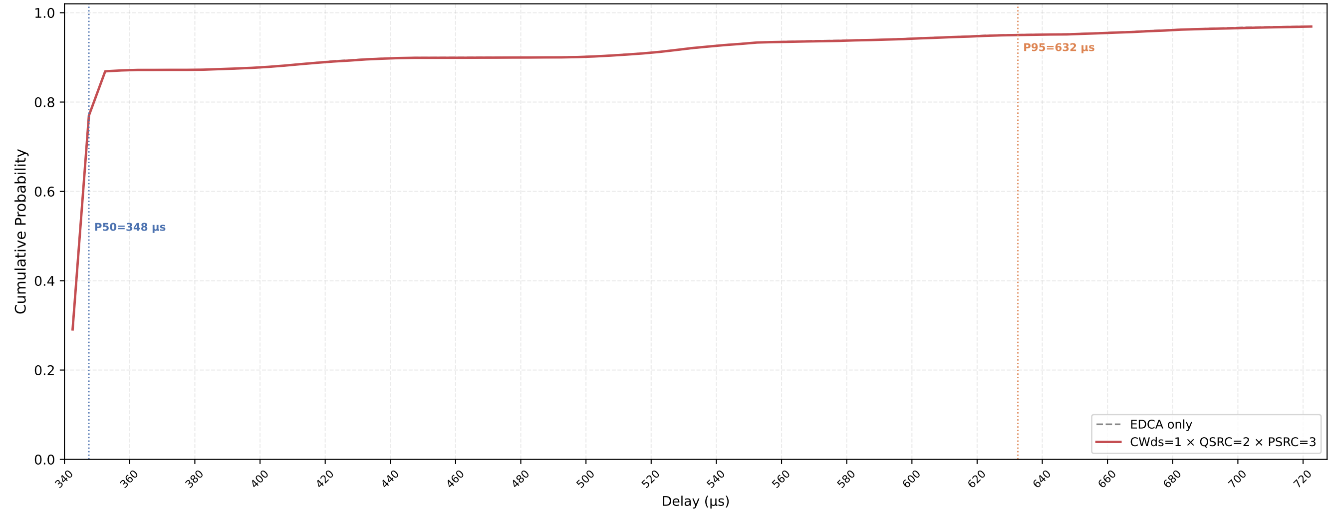
P-EDCA STA VO Delay CDF — CWds=1 × QSRC=2 × PSRC=3 nSta=30, nPedca=30, 0.1Mbps, avg of 10 runs
