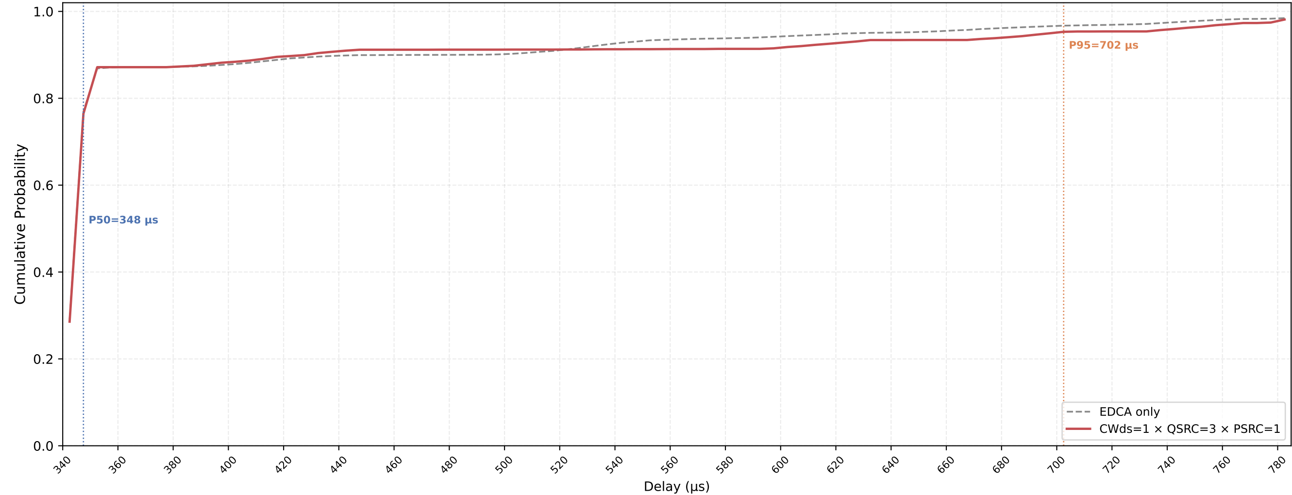
P-EDCA STA VO Delay CDF — CWds=1 × QSRC=3 × PSRC=1 nSta=30, nPedca=5, 0.1Mbps, avg of 10 runs
