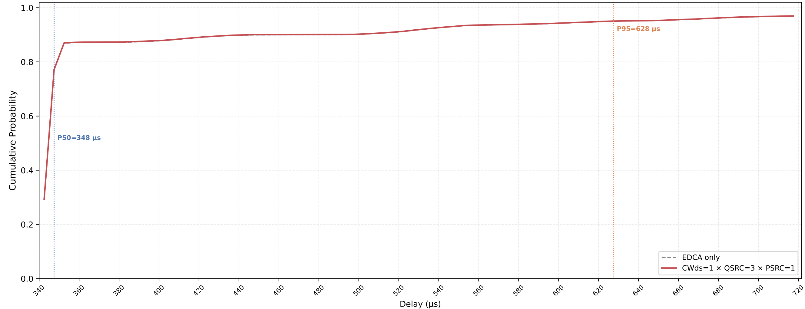
VO (all STAs) Delay CDF — CWds=1 × QSRC=3 × PSRC=1 nSta=30, nPedca=15, 0.1Mbps, avg of 10 runs
