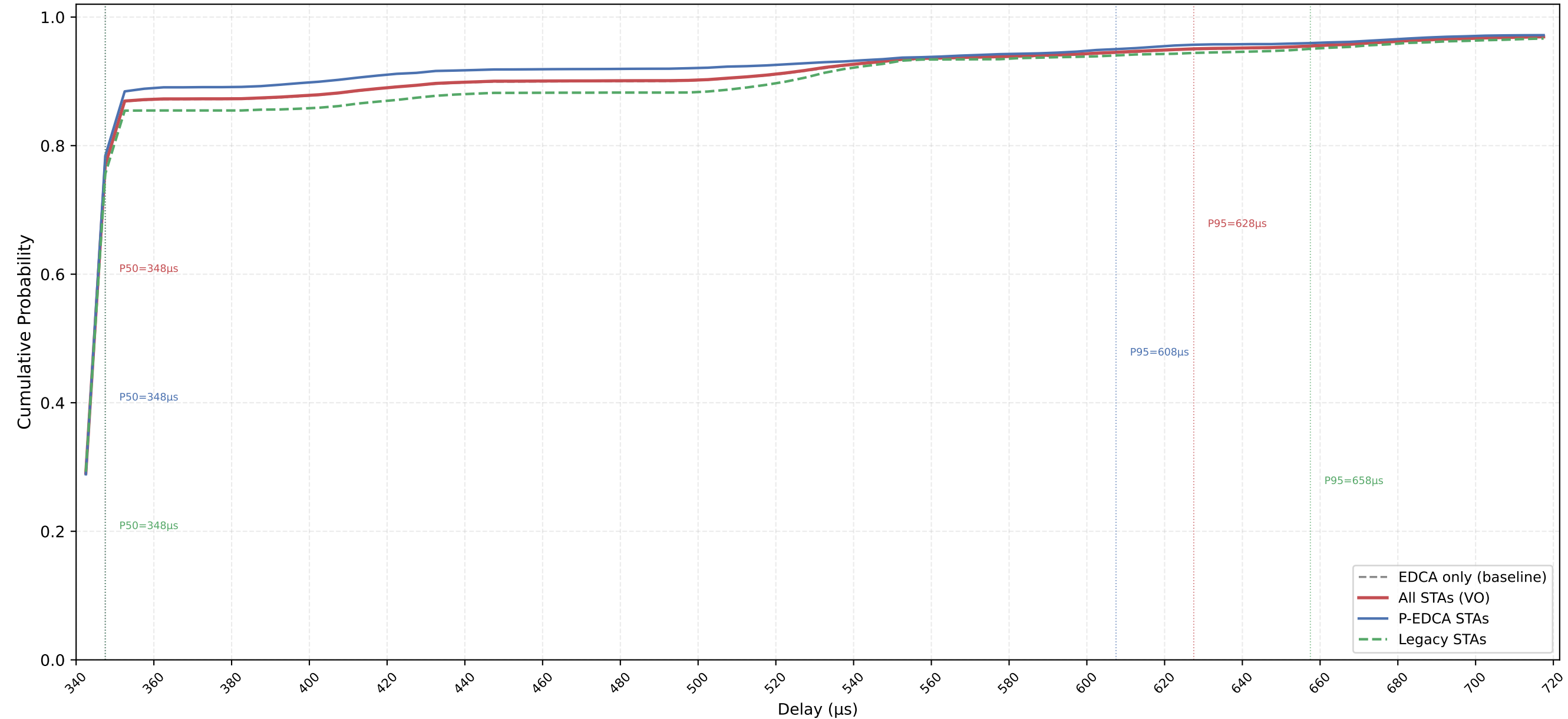
VO Delay CDF — P-EDCA / Legacy / All | CWds=1 × QSRC=3 × PSRC=2 nSta=30, nPedca=15/30, 0.1Mbps, avg of 10 runs
