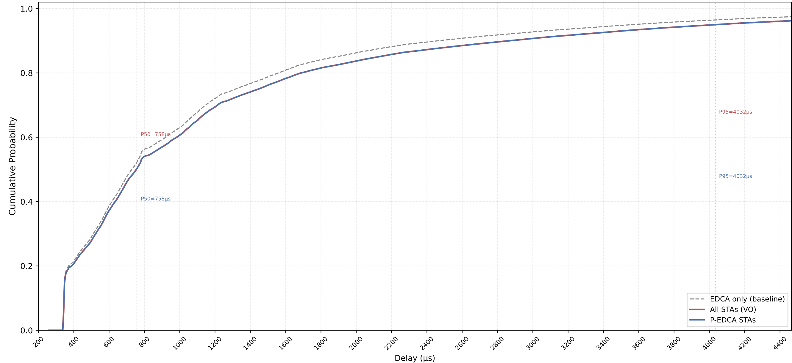
VO Delay CDF — P-EDCA / Legacy / All | CWds=1 × QSRC=3 × PSRC=2 nSta=30, nPedca=30/30, 0.5Mbps, avg of 10 runs
