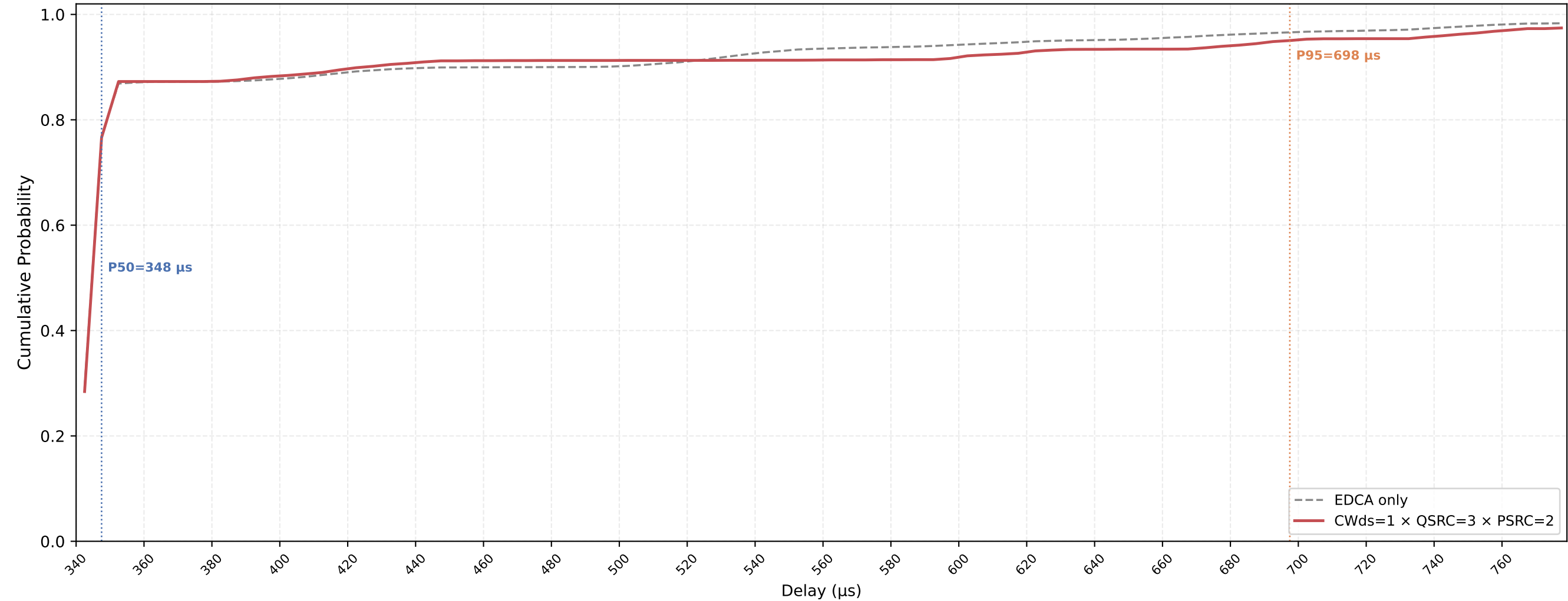
P-EDCA STA VO Delay CDF — CWds=1 × QSRC=3 × PSRC=2 nSta=30, nPedca=5, 0.1Mbps, avg of 10 runs
