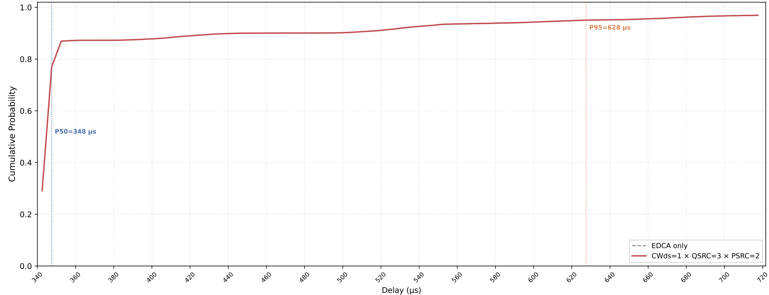
VO (all STAs) Delay CDF — CWds=1 × QSRC=3 × PSRC=2 nSta=30, nPedca=15, 0.1Mbps, avg of 10 runs
