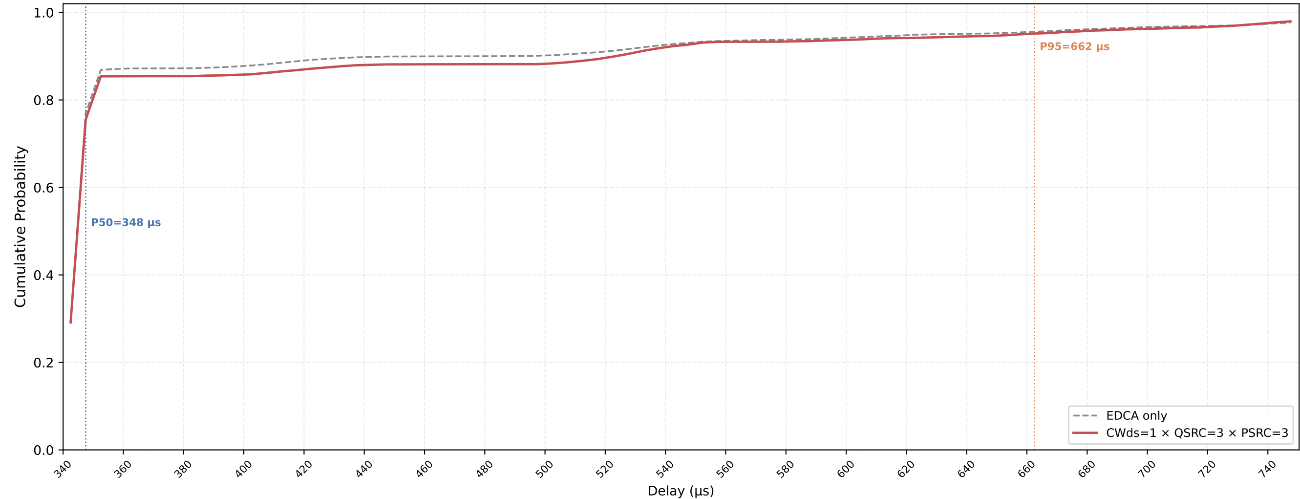
Legacy STA VO Delay CDF — CWds=1 × QSRC=3 × PSRC=3 nSta=30, nPedca=15, 0.1Mbps, avg of 10 runs
