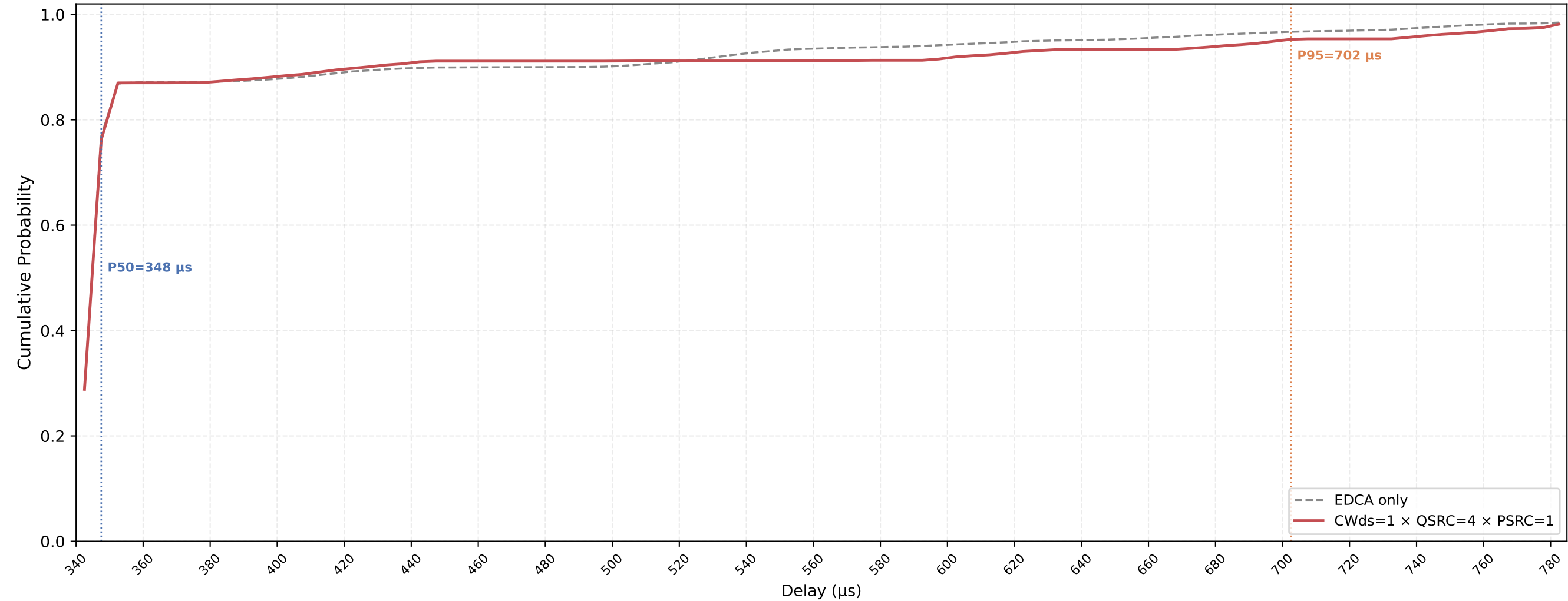
P-EDCA STA VO Delay CDF — CWds=1 × QSRC=4 × PSRC=1 nSta=30, nPedca=5, 0.1Mbps, avg of 10 runs
