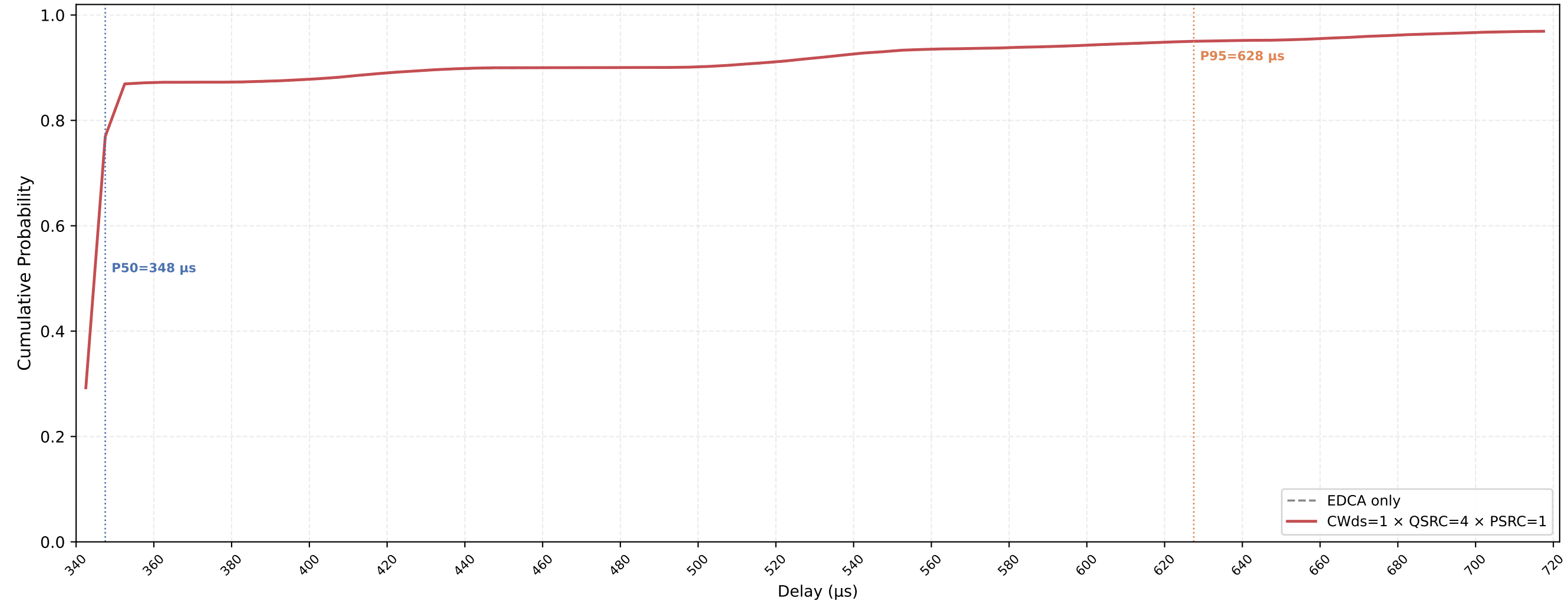
VO (all STAs) Delay CDF — CWds=1 × QSRC=4 × PSRC=1 nSta=30, nPedca=5, 0.1Mbps, avg of 10 runs
