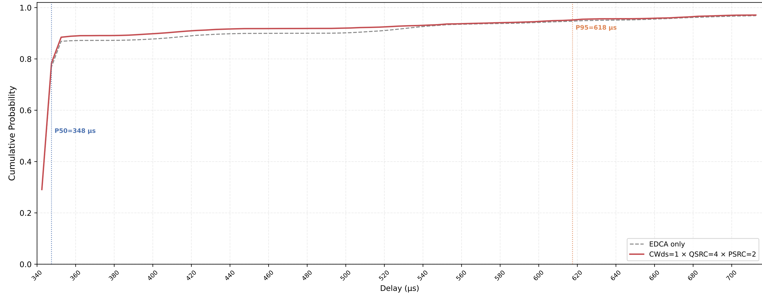
P-EDCA STA VO Delay CDF — CWds=1 × QSRC=4 × PSRC=2 nSta=30, nPedca=15, 0.1Mbps, avg of 10 runs
