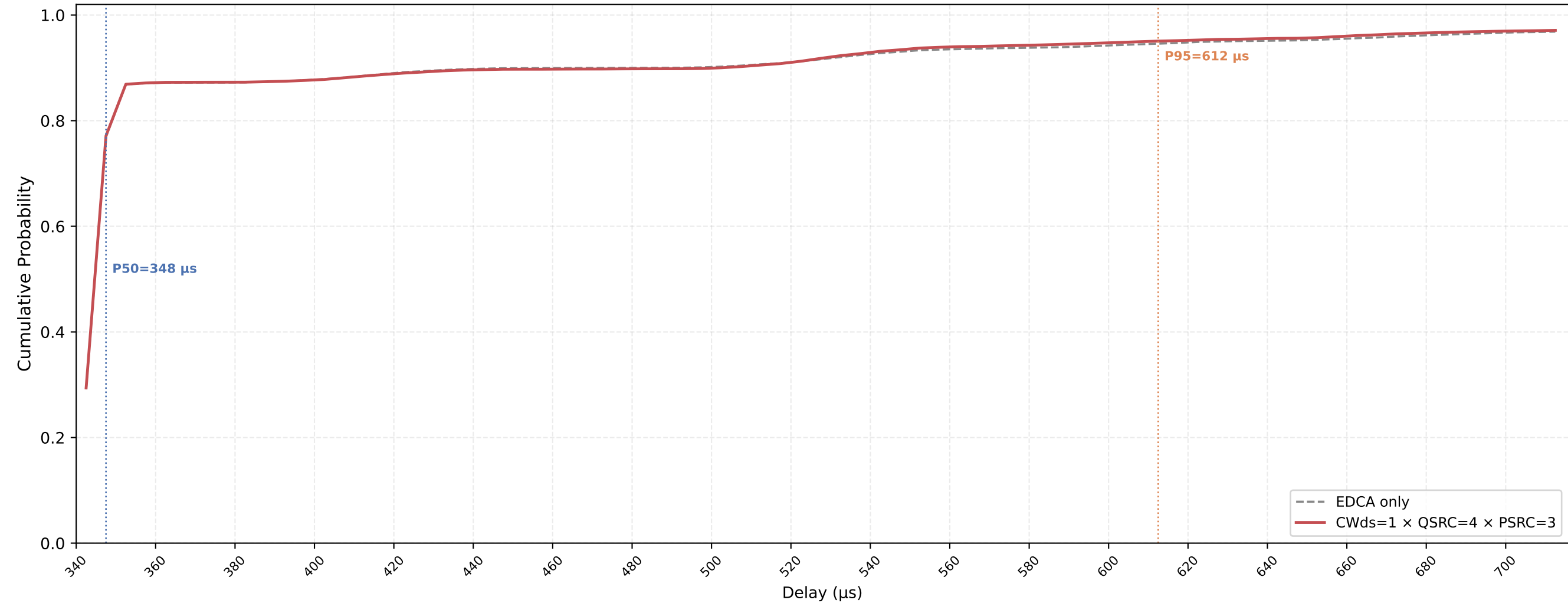
Legacy STA VO Delay CDF — CWds=1 × QSRC=4 × PSRC=3 nSta=30, nPedca=5, 0.1Mbps, avg of 10 runs
