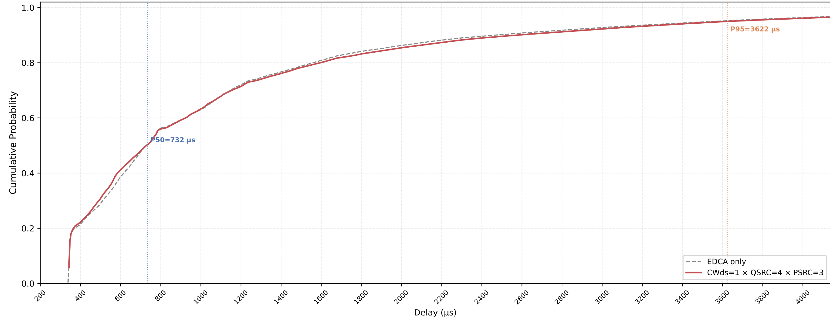
P-EDCA STA VO Delay CDF — CWds=1 × QSRC=4 × PSRC=3 nSta=30, nPedca=15, 0.5Mbps, avg of 10 runs
