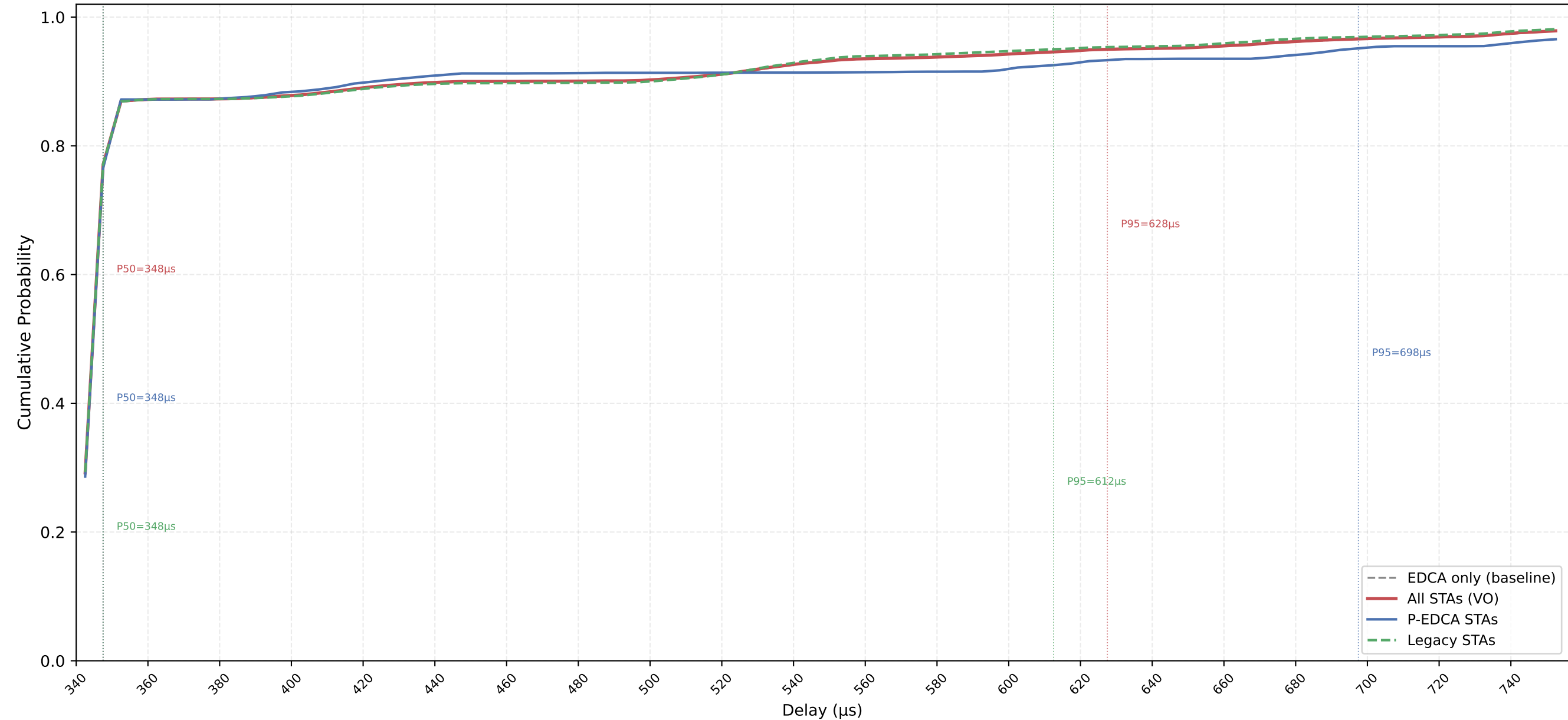
VO Delay CDF — P-EDCA / Legacy / All | CWds=1 × QSRC=5 × PSRC=1 nSta=30, nPedca=5/30, 0.1Mbps, avg of 10 runs
