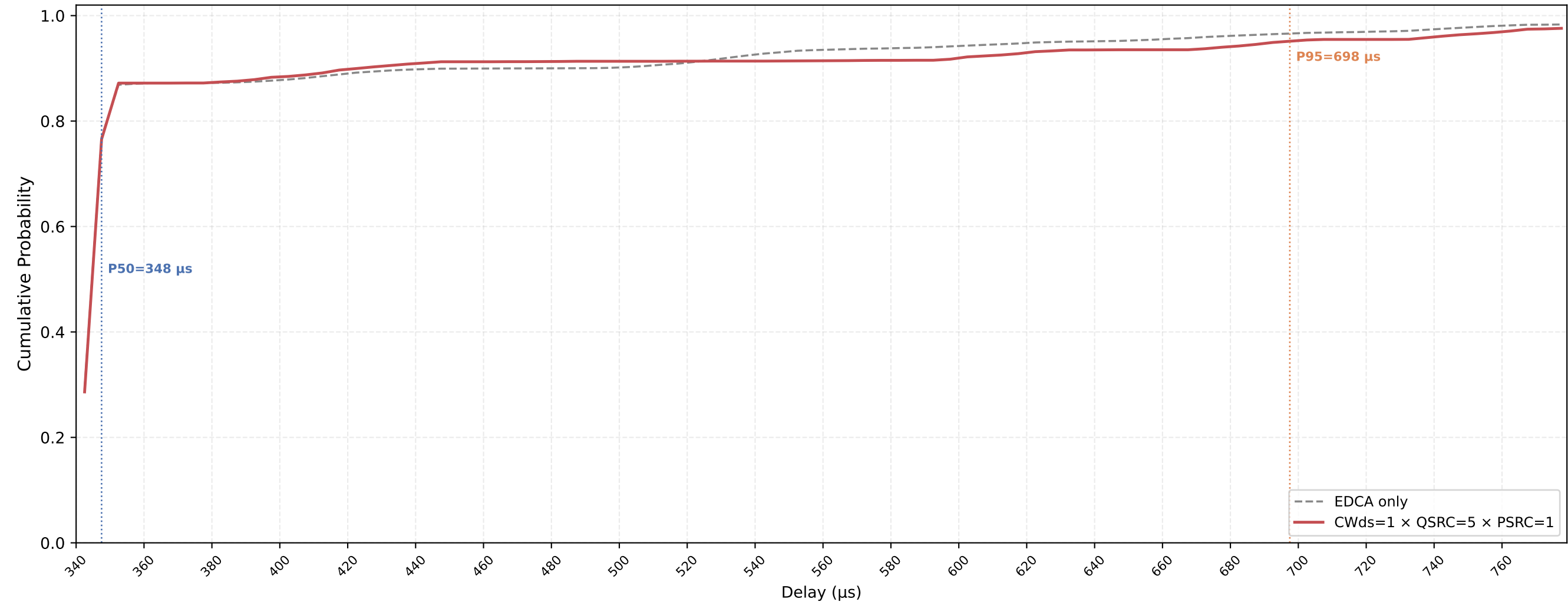
P-EDCA STA VO Delay CDF — CWds=1 × QSRC=5 × PSRC=1 nSta=30, nPedca=5, 0.1Mbps, avg of 10 runs
