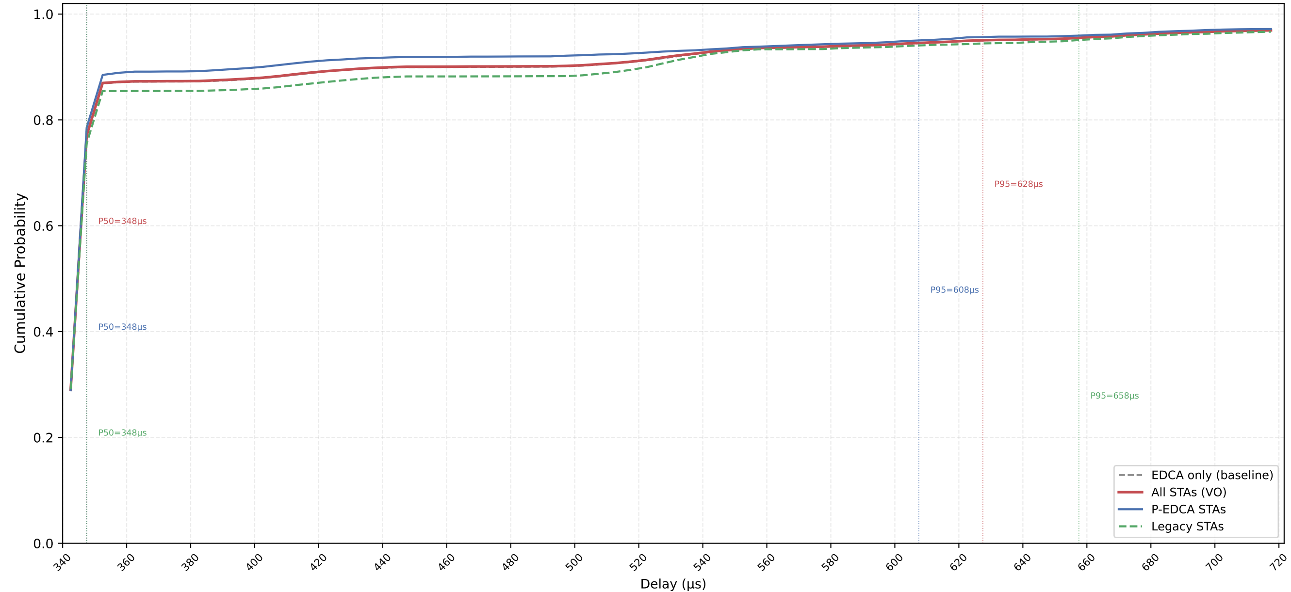
VO Delay CDF — P-EDCA / Legacy / All | CWds=1 × QSRC=5 × PSRC=3 nSta=30, nPedca=15/30, 0.1Mbps, avg of 10 runs
