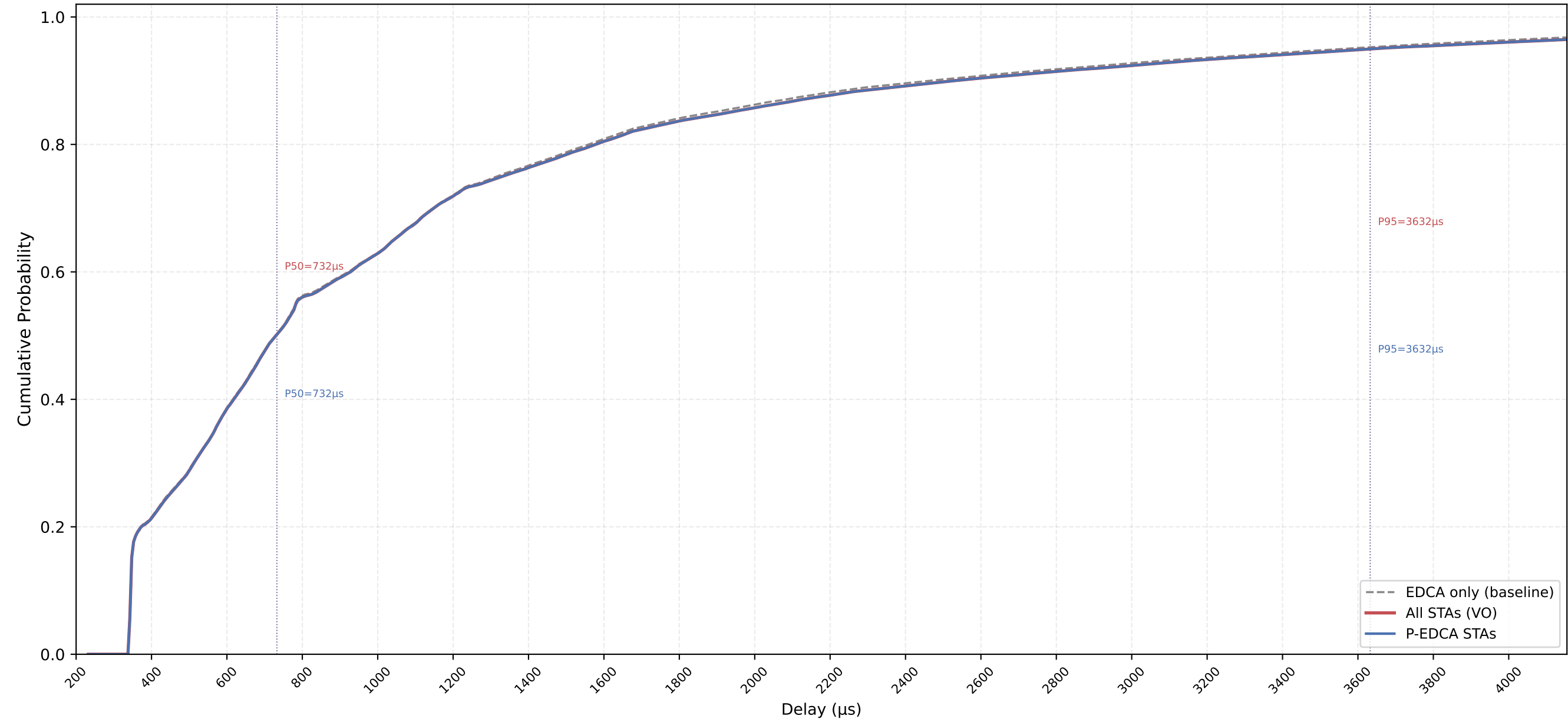
VO Delay CDF — P-EDCA / Legacy / All | CWds=1 × QSRC=5 × PSRC=3 nSta=30, nPedca=30/30, 0.5Mbps, avg of 10 runs
