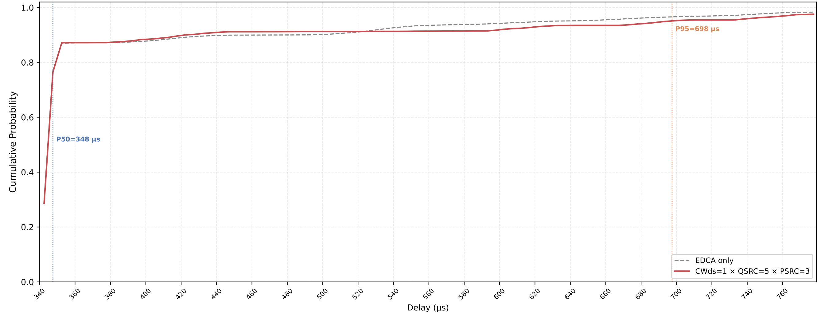
P-EDCA STA VO Delay CDF — CWds=1 × QSRC=5 × PSRC=3 nSta=30, nPedca=5, 0.1Mbps, avg of 10 runs
