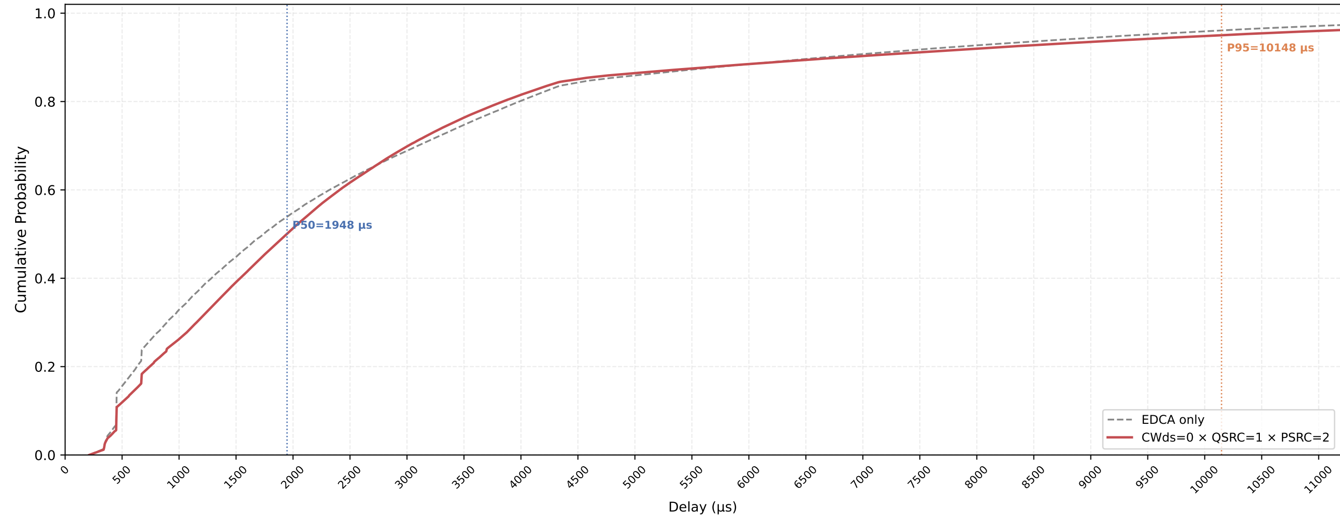
VO (all STAs) Delay CDF — CWds=0 × QSRC=1 × PSRC=2 nSta=30, nPedca=30, 1Mbps, avg of 10 runs
