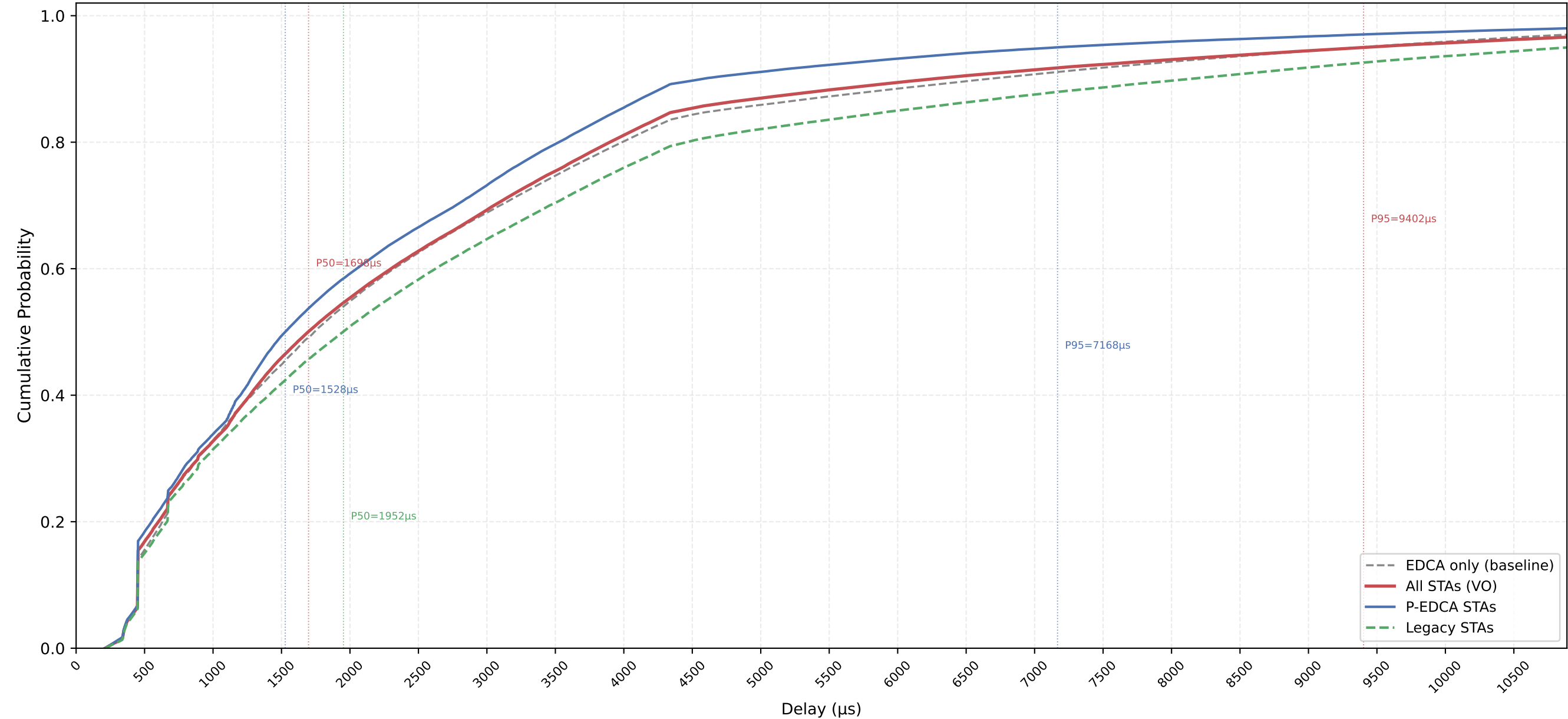
VO Delay CDF — P-EDCA / Legacy / All | CWds=0 × QSRC=3 × PSRC=2 nSta=30, nPedca=15/30, 1Mbps, avg of 10 runs
