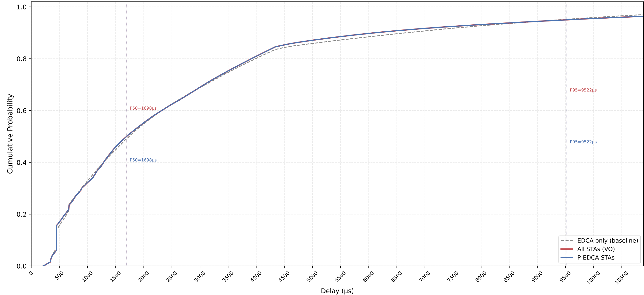
VO Delay CDF — P-EDCA / Legacy / All | CWds=0 × QSRC=3 × PSRC=2 nSta=30, nPedca=30/30, 1Mbps, avg of 10 runs
