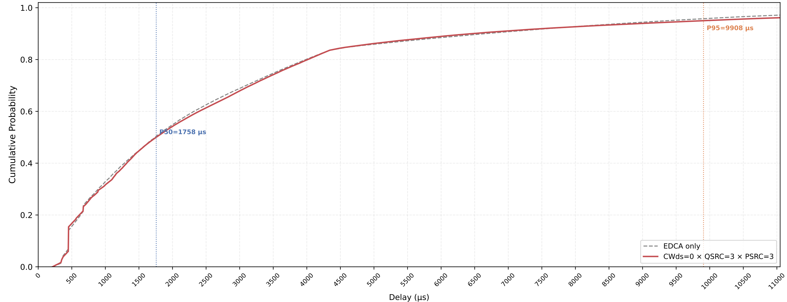
VO (all STAs) Delay CDF — CWds=0 × QSRC=3 × PSRC=3 nSta=30, nPedca=30, 1Mbps, avg of 10 runs
