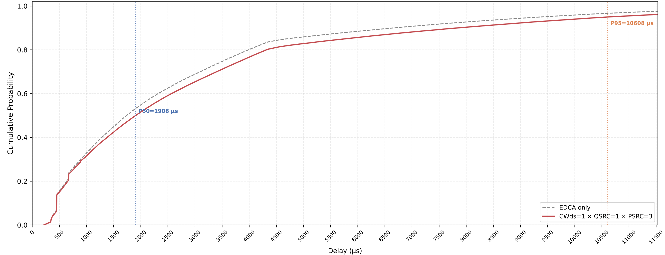
Legacy STA VO Delay CDF — CWds=1 × QSRC=1 × PSRC=3 nSta=30, nPedca=5, 1Mbps, avg of 10 runs
