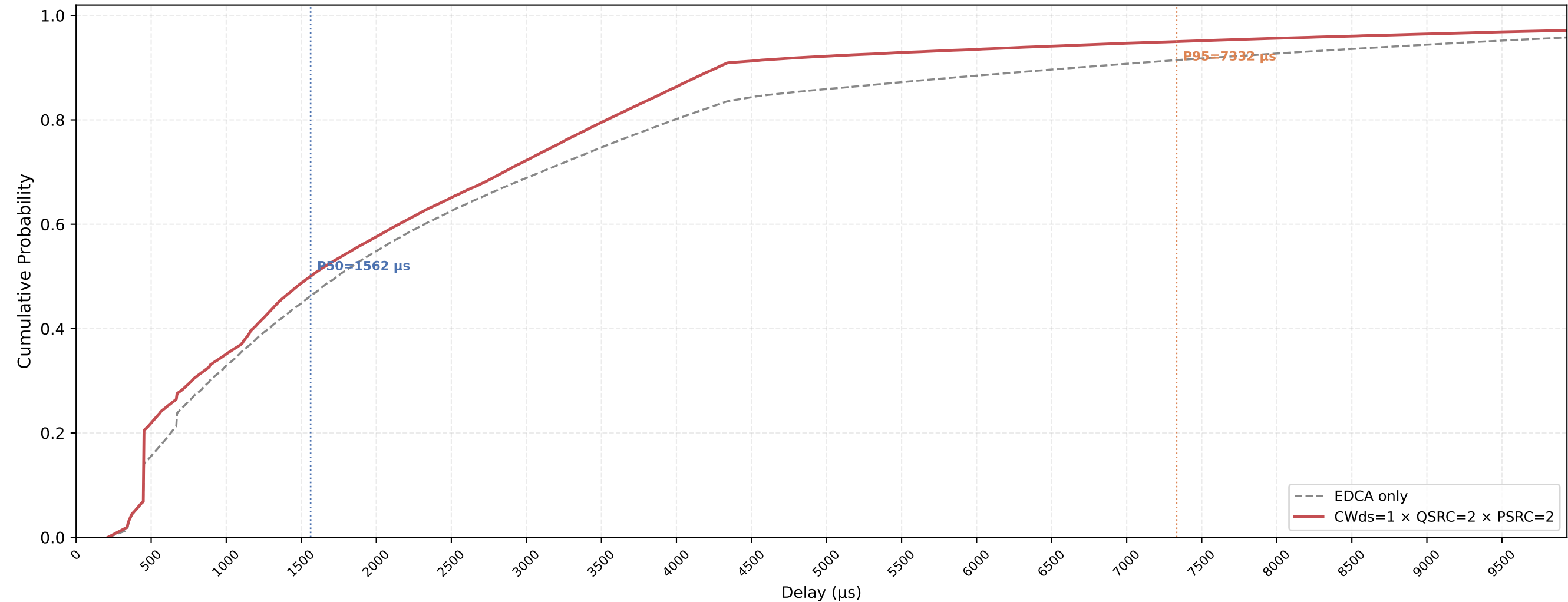
P-EDCA STA VO Delay CDF — CWds=1 × QSRC=2 × PSRC=2 nSta=30, nPedca=15, 1Mbps, avg of 10 runs
