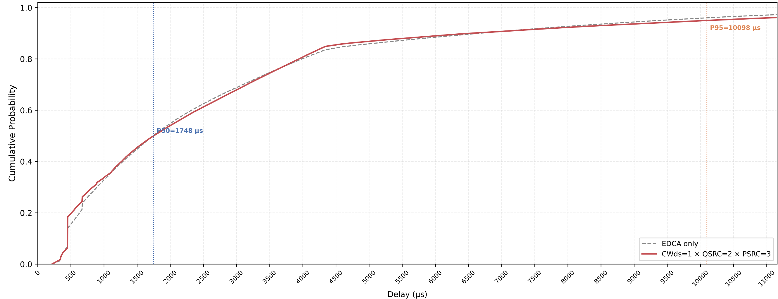
VO (all STAs) Delay CDF — CWds=1 × QSRC=2 × PSRC=3 nSta=30, nPedca=15, 1Mbps, avg of 10 runs
