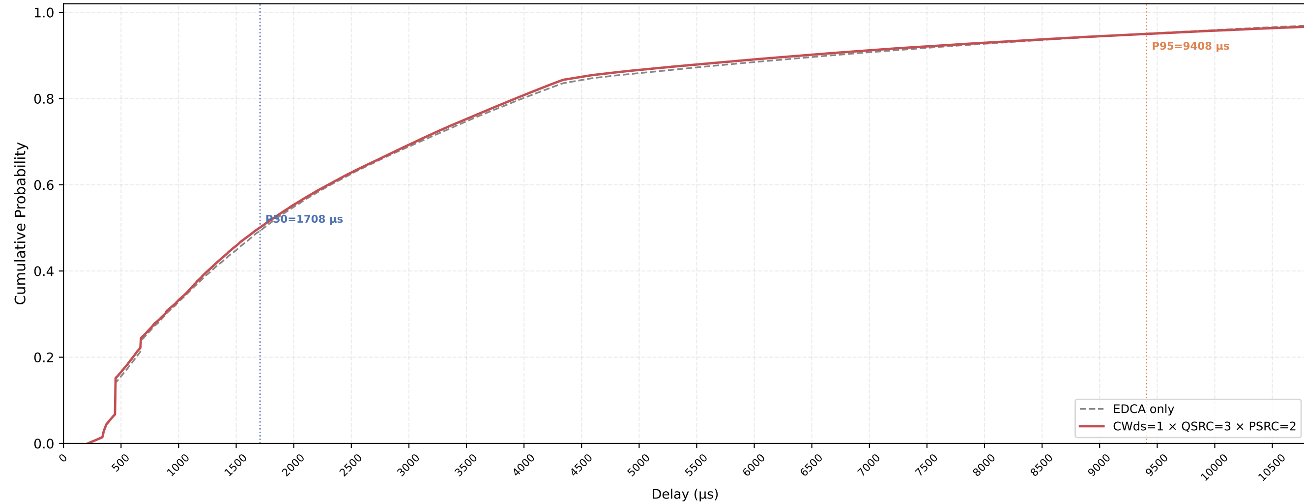
VO (all STAs) Delay CDF — CWds=1 × QSRC=3 × PSRC=2 nSta=30, nPedca=5, 1Mbps, avg of 10 runs
