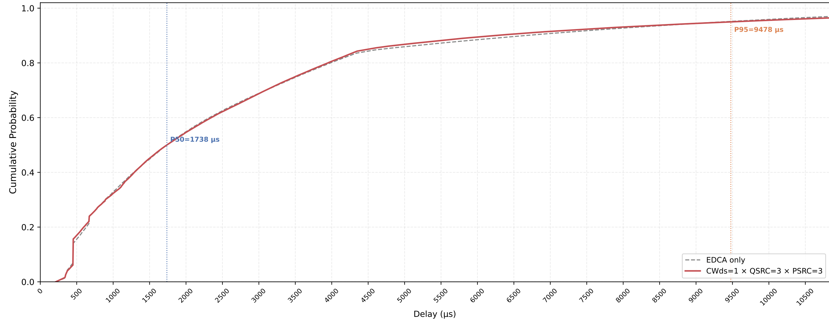
VO (all STAs) Delay CDF — CWds=1 × QSRC=3 × PSRC=3 nSta=30, nPedca=15, 1Mbps, avg of 10 runs
