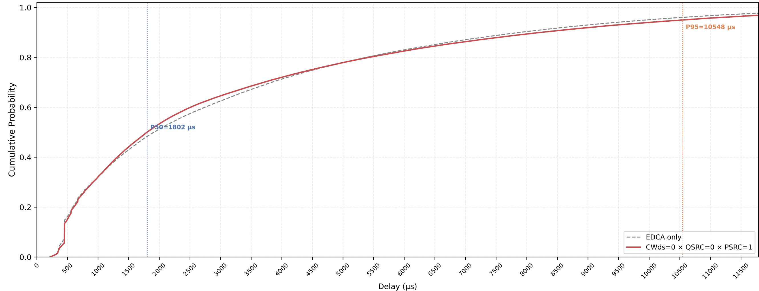
VO (all STAs) Delay CDF — CWds=0 × QSRC=0 × PSRC=1 nSta=30, nPedca=5, 1Mbps, avg of 10 runs
