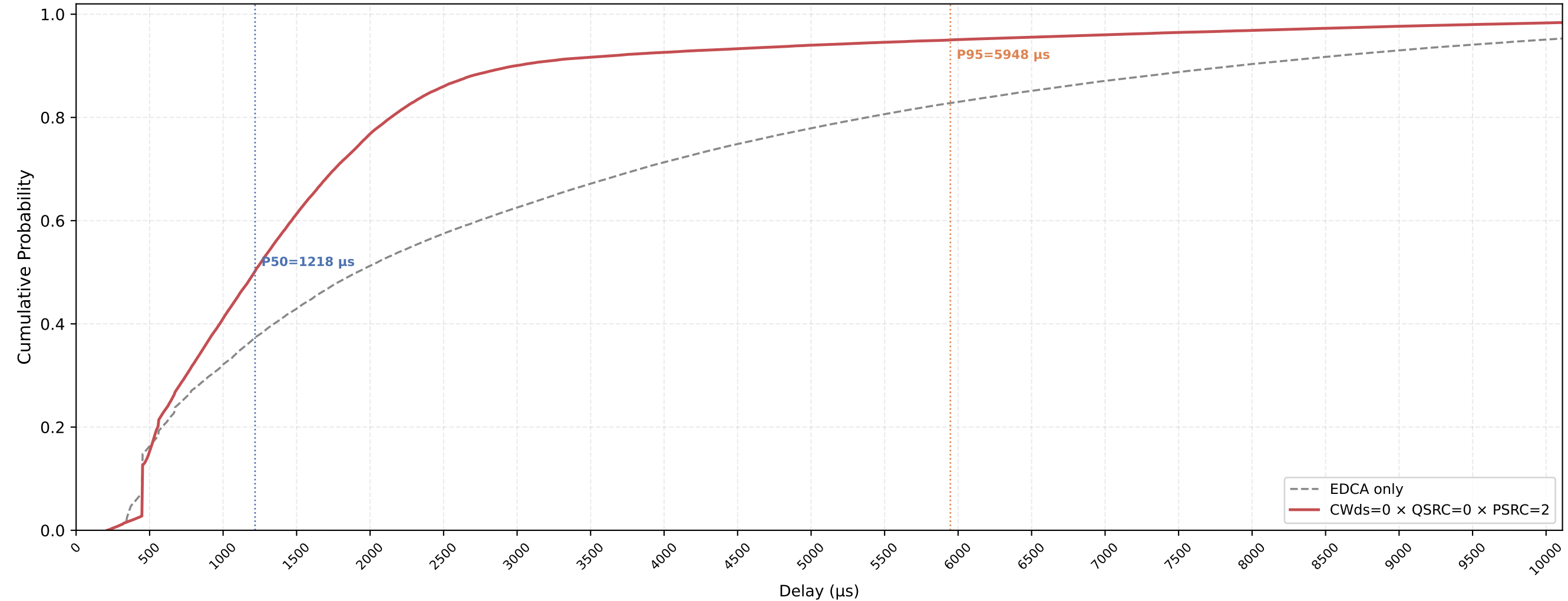
P-EDCA STA VO Delay CDF — CWds=0 × QSRC=0 × PSRC=2 nSta=30, nPedca=5, 1Mbps, avg of 10 runs
